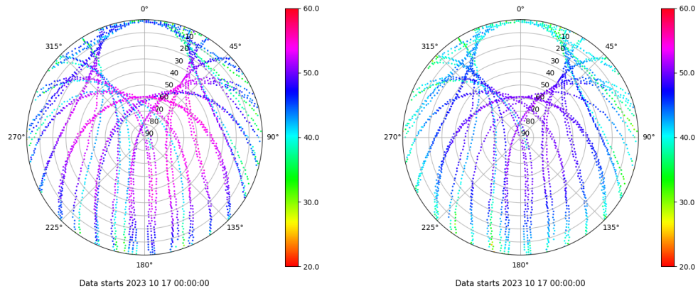
Skyplot for station VALA. Signal to Noise S1C Data file VALA00ESP_R_2023290.xtr Skyplot for station VALA. Signal to Noise S2C Data file VALA00ESP_R_2023290.xtr
