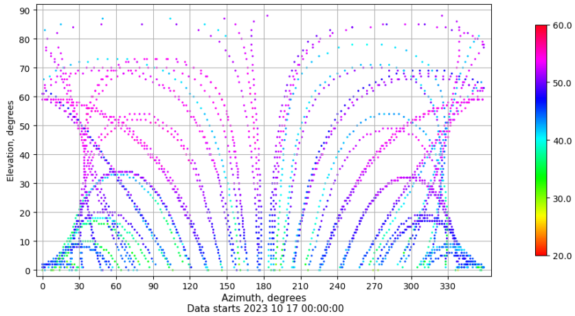
Azimuth-elevation plot for station VALA. Signal to Noise S1C Data file VALA00ESP_R_2023290.xtr
