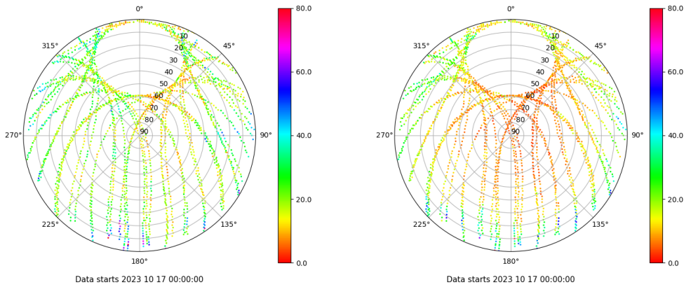
Skyplot for station VALA. Parameter M1C Data file VALA00ESP_R_2023290.xtr Skyplot for station VALA. Parameter M2C Data file VALA00ESP_R_2023290.xtr
