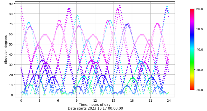
Time-elevation plot for station VALA. Signal to Noise S1C Data file VALA00ESP_R_2023290.xtr
