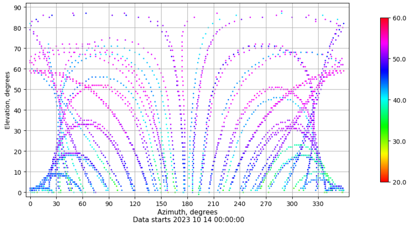
Azimuth-elevation plot for station VALA. Signal to Noise S1C Data file VALA00ESP_R_2023287.xtr
