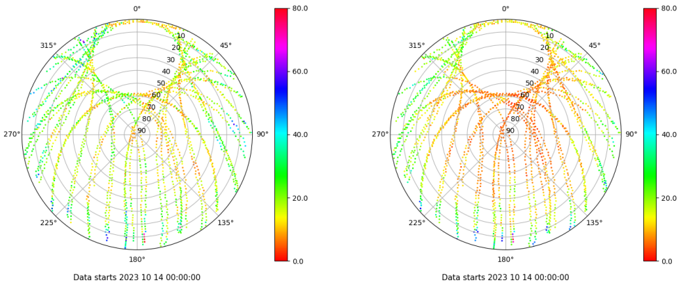
Skyplot for station VALA. Parameter M1C Data file VALA00ESP_R_2023287.xtr Skyplot for station VALA. Parameter M2C Data file VALA00ESP_R_2023287.xtr
