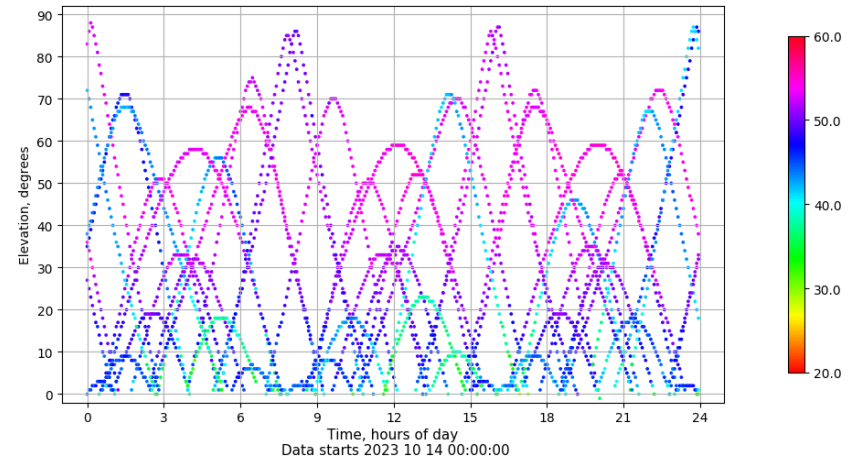
Time-elevation plot for station VALA. Signal to Noise S1C Data file VALA00ESP_R_2023287.xtr
