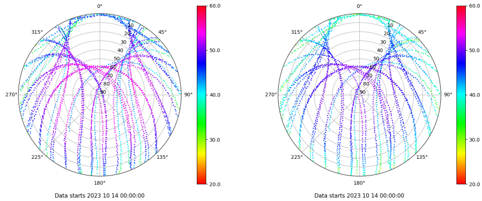
Skyplot for station VALA. Signal to Noise S1C Data file VALA00ESP_R_2023287.xtr Skyplot for station VALA. Signal to Noise S2C Data file VALA00ESP_R_2023287.xtr
