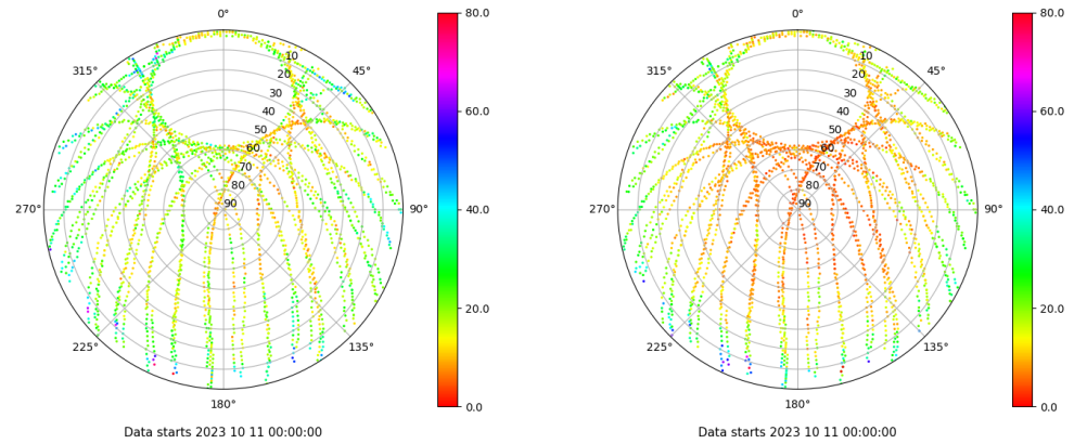
Skyplot for station VALA. Parameter M1C Data file VALA00ESP_R_2023284.xtr Skyplot for station VALA. Parameter M2C Data file VALA00ESP_R_2023284.xtr
