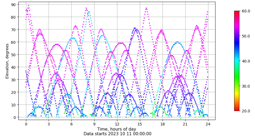
Time-elevation plot for station VALA. Signal to Noise S1C Data file VALA00ESP_R_2023284.xtr
