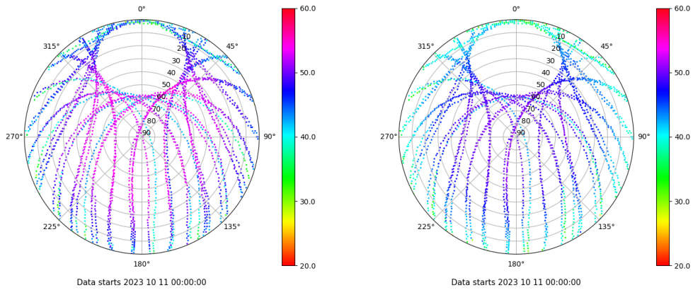
Skyplot for station VALA. Signal to Noise S1C Data file VALA00ESP_R_2023284.xtr Skyplot for station VALA. Signal to Noise S2C Data file VALA00ESP_R_2023284.xtr
