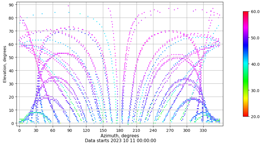
Azimuth-elevation plot for station VALA. Signal to Noise S1C Data file VALA00ESP_R_2023284.xtr
