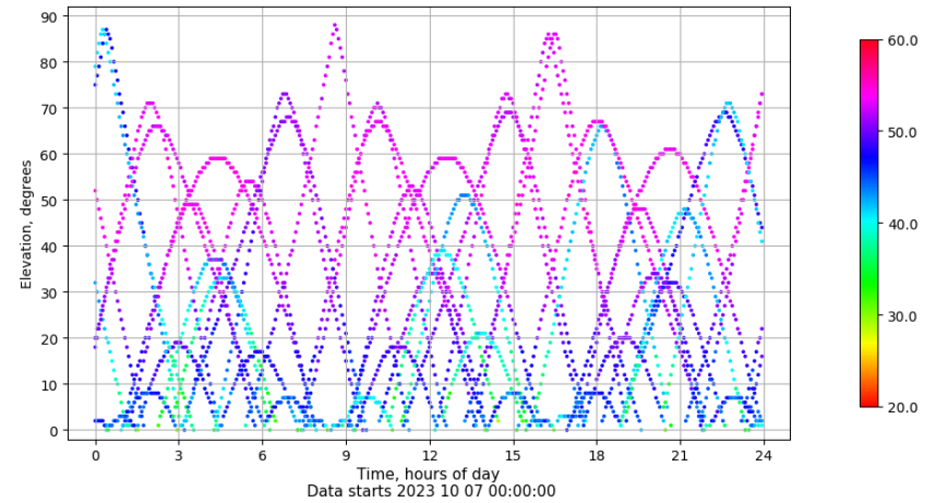
Time-elevation plot for station VALA. Signal to Noise S1C Data file VALA00ESP_R_2023280.xtr
