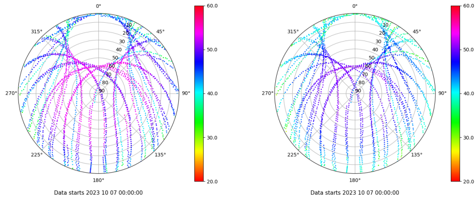
Skyplot for station VALA. Signal to Noise S1C Data file VALA00ESP_R_2023280.xtr Skyplot for station VALA. Signal to Noise S2C Data file VALA00ESP_R_2023280.xtr
