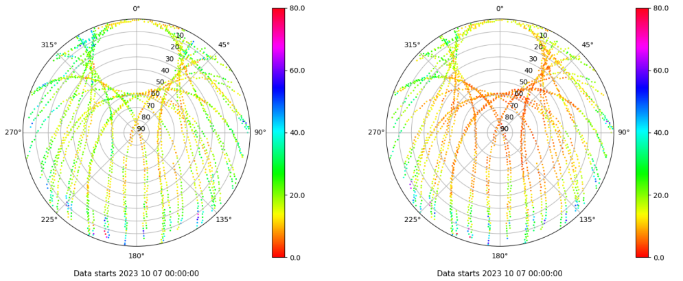
Skyplot for station VALA. Parameter M1C Data file VALA00ESP_R_2023280.xtr Skyplot for station VALA. Parameter M2C Data file VALA00ESP_R_2023280.xtr
