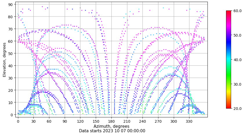
Azimuth-elevation plot for station VALA. Signal to Noise S1C Data file VALA00ESP_R_2023280.xtr
