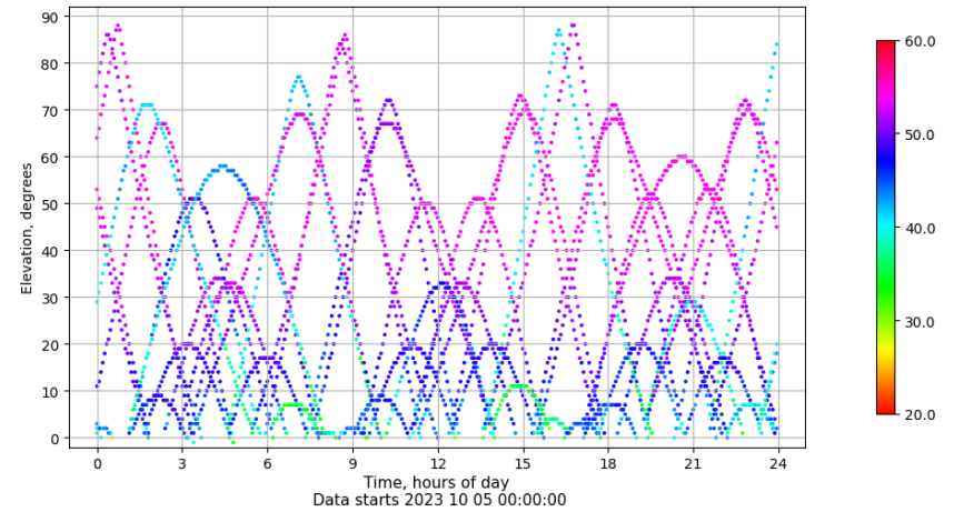
Time-elevation plot for station VALA. Signal to Noise S1C Data file VALA00ESP_R_2023278.xtr
