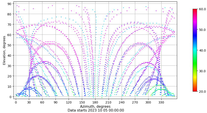
Azimuth-elevation plot for station VALA. Signal to Noise S1C Data file VALA00ESP_R_2023278.xtr
