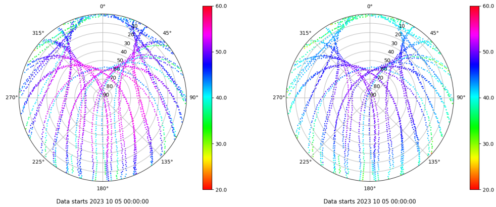
Skyplot for station VALA. Signal to Noise S1C Data file VALA00ESP_R_2023278.xtr Skyplot for station VALA. Signal to Noise S2C Data file VALA00ESP_R_2023278.xtr
