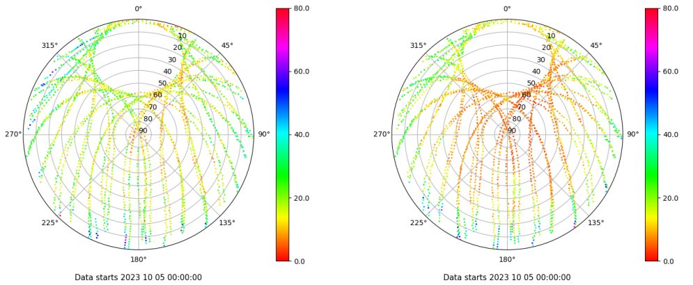
Skyplot for station VALA. Parameter M1C Data file VALA00ESP_R_2023278.xtr Skyplot for station VALA. Parameter M2C Data file VALA00ESP_R_2023278.xtr
