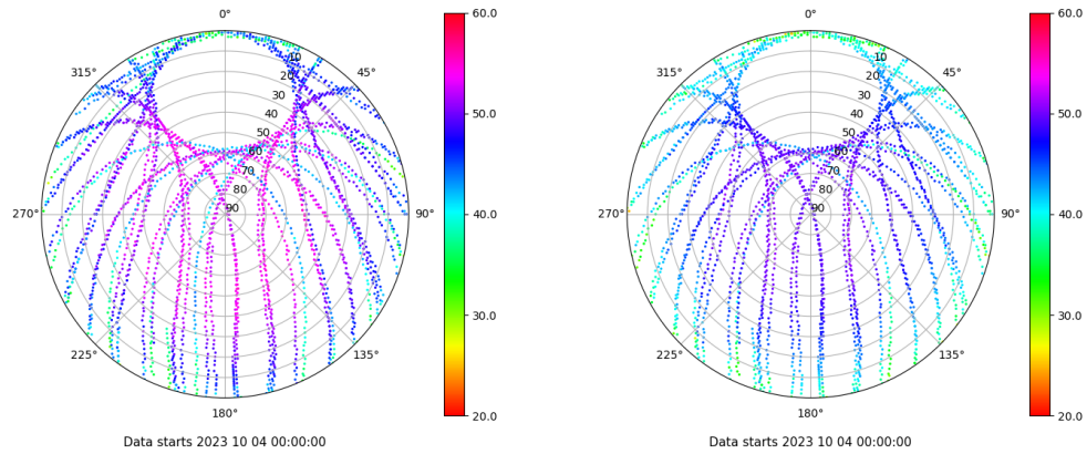
Skyplot for station VALA. Signal to Noise S1C Data file VALA00ESP_R_2023277.xtr Skyplot for station VALA. Signal to Noise S2C Data file VALA00ESP_R_2023277.xtr
