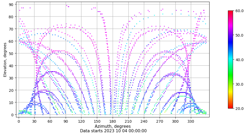
Azimuth-elevation plot for station VALA. Signal to Noise S1C Data file VALA00ESP_R_2023277.xtr
