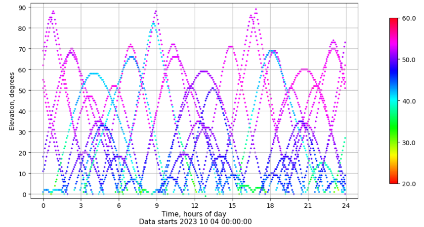
Time-elevation plot for station VALA. Signal to Noise S1C Data file VALA00ESP_R_2023277.xtr
