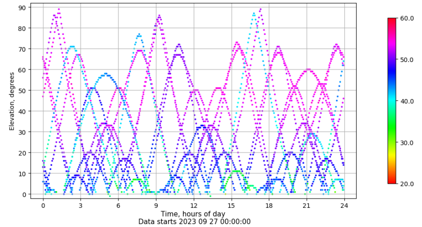
Time-elevation plot for station VALA. Signal to Noise S1C Data file VALA00ESP_R_2023270.xtr
