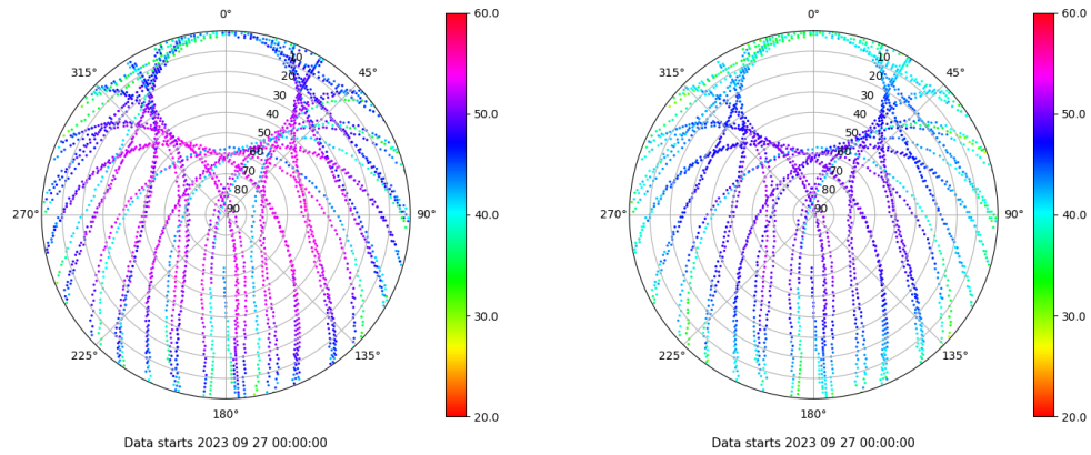
Skyplot for station VALA. Signal to Noise S1C Data file VALA00ESP_R_2023270.xtr Skyplot for station VALA. Signal to Noise S2C Data file VALA00ESP_R_2023270.xtr
