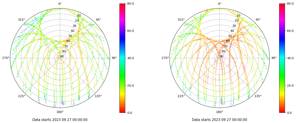
Skyplot for station VALA. Parameter M1C Data file VALA00ESP_R_2023270.xtr Skyplot for station VALA. Parameter M2C Data file VALA00ESP_R_2023270.xtr
