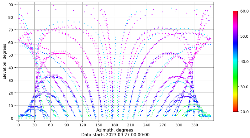
Azimuth-elevation plot for station VALA. Signal to Noise S1C Data file VALA00ESP_R_2023270.xtr
