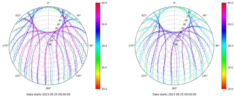
Skyplot for station VALA. Signal to Noise S1C Data file VALA00ESP_R_2023268.xtr Skyplot for station VALA. Signal to Noise S2C Data file VALA00ESP_R_2023268.xtr
