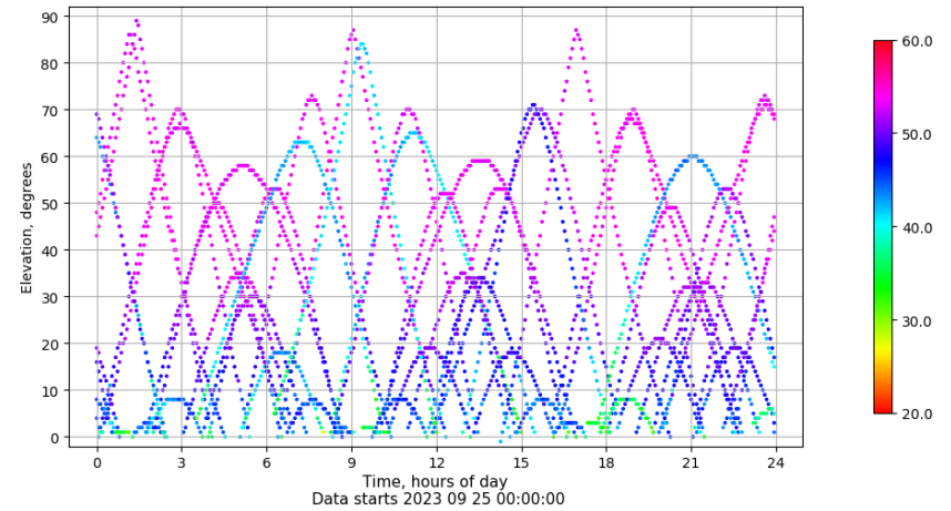
Time-elevation plot for station VALA. Signal to Noise S1C Data file VALA00ESP_R_2023268.xtr
