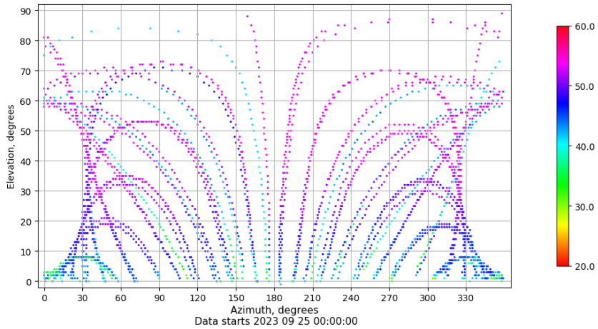
Azimuth-elevation plot for station VALA. Signal to Noise S1C Data file VALA00ESP_R_2023268.xtr
