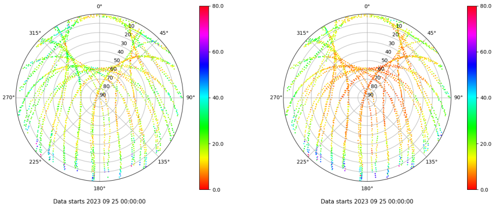
Skyplot for station VALA. Parameter M1C Data file VALA00ESP_R_2023268.xtr Skyplot for station VALA. Parameter M2C Data file VALA00ESP_R_2023268.xtr
