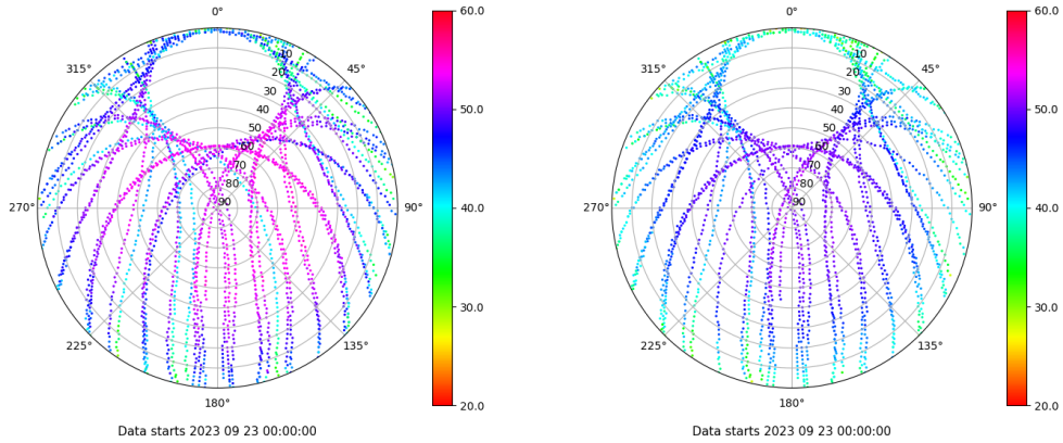
Skyplot for station VALA. Signal to Noise S1C Data file VALA00ESP_R_2023266.xtr Skyplot for station VALA. Signal to Noise S2C Data file VALA00ESP_R_2023266.xtr
