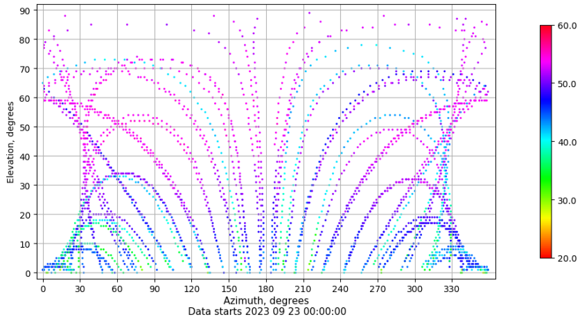
Azimuth-elevation plot for station VALA. Signal to Noise S1C Data file VALA00ESP_R_2023266.xtr
