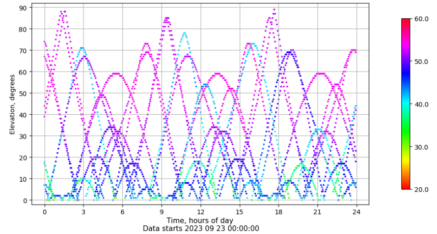
Time-elevation plot for station VALA. Signal to Noise S1C Data file VALA00ESP_R_2023266.xtr
