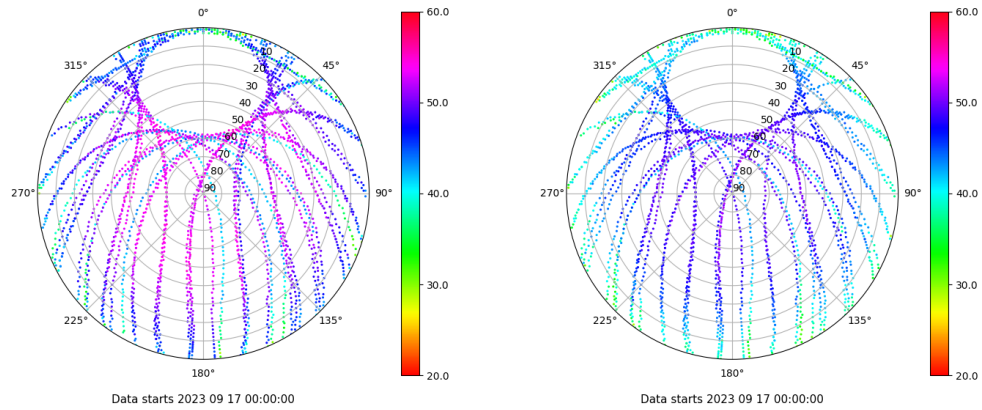
Skyplot for station VALA. Signal to Noise S1C Data file VALA00ESP_R_2023260.xtr Skyplot for station VALA. Signal to Noise S2C Data file VALA00ESP_R_2023260.xtr
