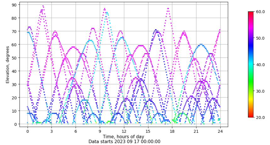
Time-elevation plot for station VALA. Signal to Noise S1C Data file VALA00ESP_R_2023260.xtr
