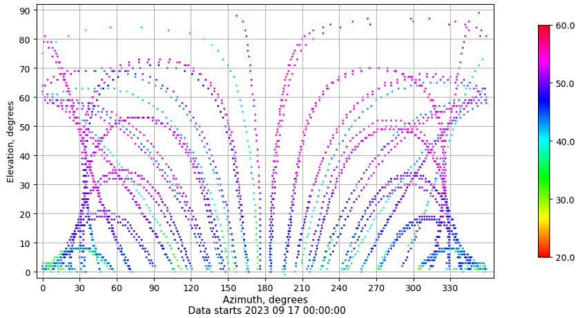
Azimuth-elevation plot for station VALA. Signal to Noise S1C Data file VALA00ESP_R_2023260.xtr
