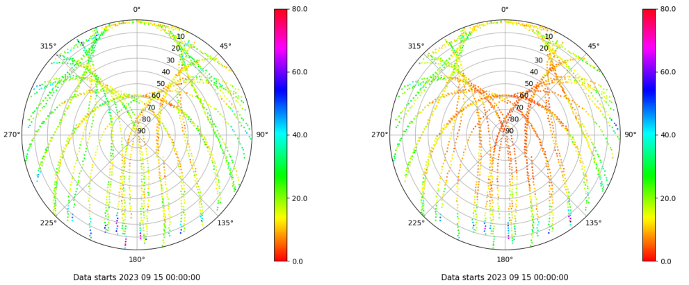
Skyplot for station VALA. Parameter M1C Data file VALA00ESP_R_2023258.xtr Skyplot for station VALA. Parameter M2C Data file VALA00ESP_R_2023258.xtr
