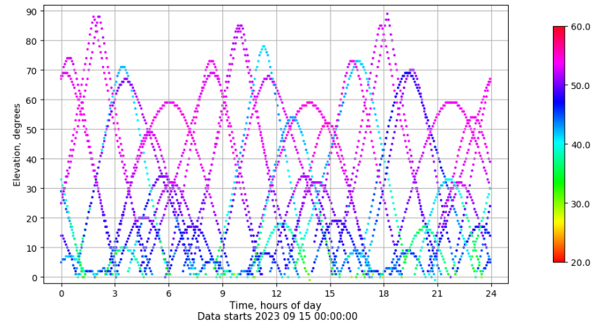
Time-elevation plot for station VALA. Signal to Noise S1C Data file VALA00ESP_R_2023258.xtr
