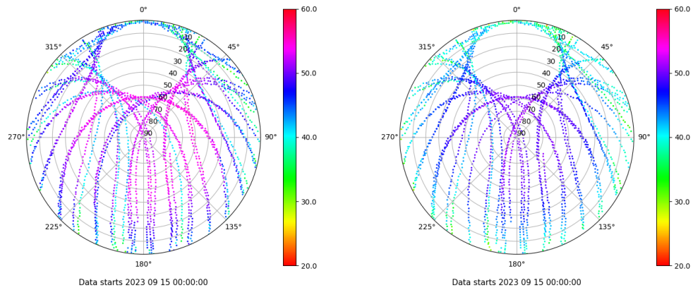
Skyplot for station VALA. Signal to Noise S1C Data file VALA00ESP_R_2023258.xtr Skyplot for station VALA. Signal to Noise S2C Data file VALA00ESP_R_2023258.xtr
