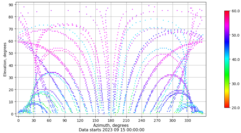
Azimuth-elevation plot for station VALA. Signal to Noise S1C Data file VALA00ESP_R_2023258.xtr
