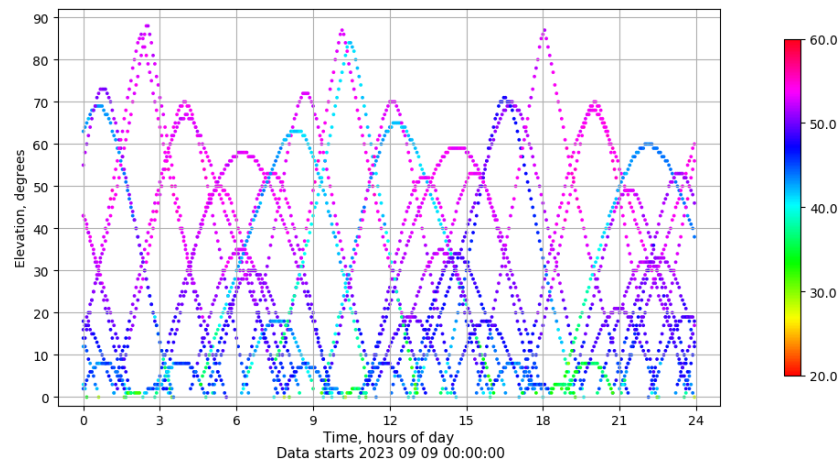
Time-elevation plot for station VALA. Signal to Noise S1C Data file VALA00ESP_R_2023252.xtr
