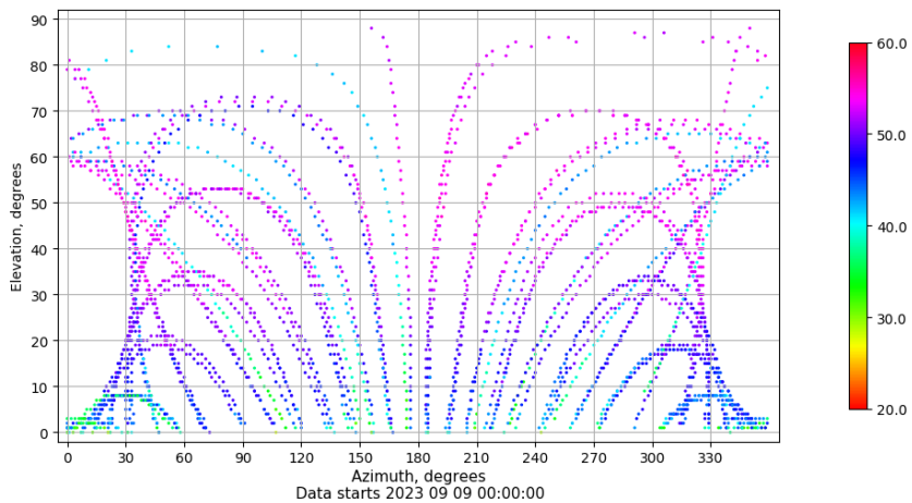
Azimuth-elevation plot for station VALA. Signal to Noise S1C Data file VALA00ESP_R_2023252.xtr
