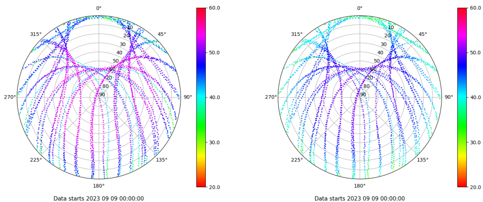
Skyplot for station VALA. Signal to Noise S1C Data file VALA00ESP_R_2023252.xtr Skyplot for station VALA. Signal to Noise S2C Data file VALA00ESP_R_2023252.xtr
