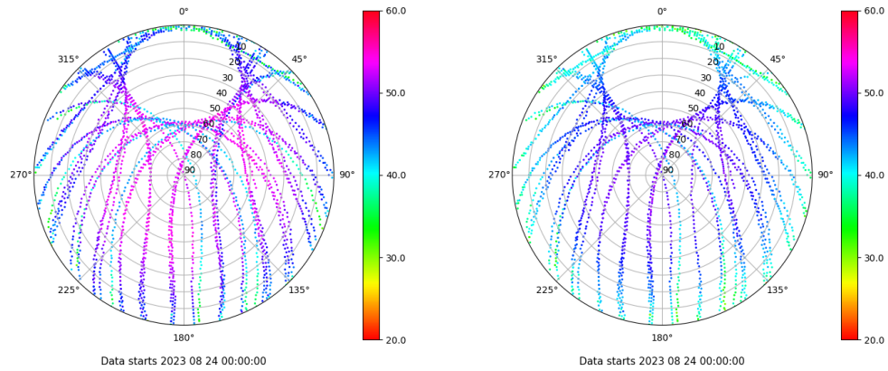
Skyplot for station VALA. Signal to Noise S1C Data file VALA00ESP_R_2023236.xtr Skyplot for station VALA. Signal to Noise S2C Data file VALA00ESP_R_2023236.xtr
