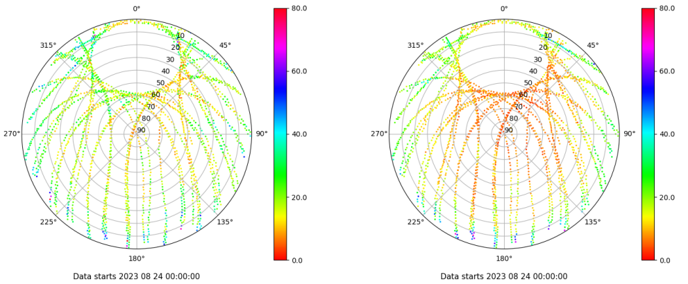
Skyplot for station VALA. Parameter M1C Data file VALA00ESP_R_2023236.xtr Skyplot for station VALA. Parameter M2C Data file VALA00ESP_R_2023236.xtr
