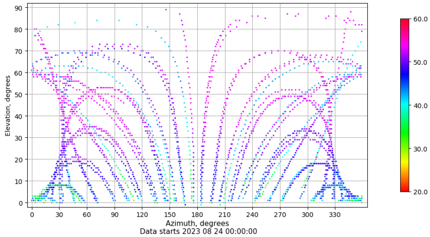
Azimuth-elevation plot for station VALA. Signal to Noise S1C Data file VALA00ESP_R_2023236.xtr
