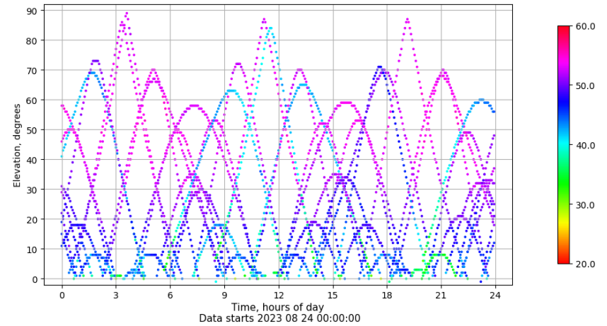
Time-elevation plot for station VALA. Signal to Noise S1C Data file VALA00ESP_R_2023236.xtr
