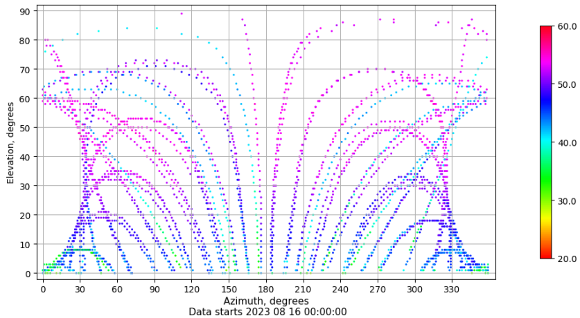
Azimuth-elevation plot for station VALA. Signal to Noise S1C Data file VALA00ESP_R_2023228.xtr
