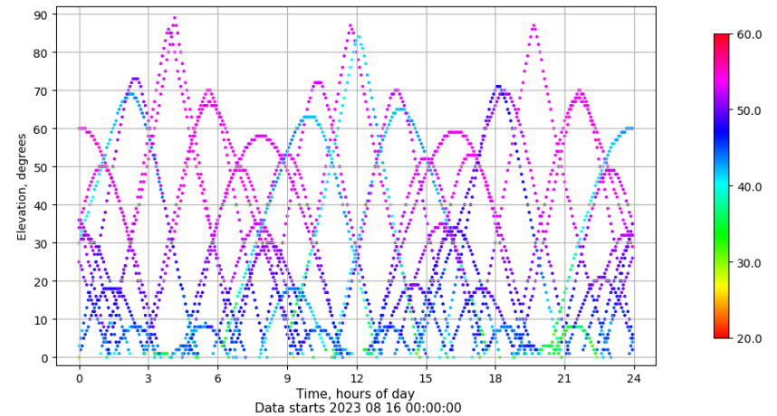
Time-elevation plot for station VALA. Signal to Noise S1C Data file VALA00ESP_R_2023228.xtr
