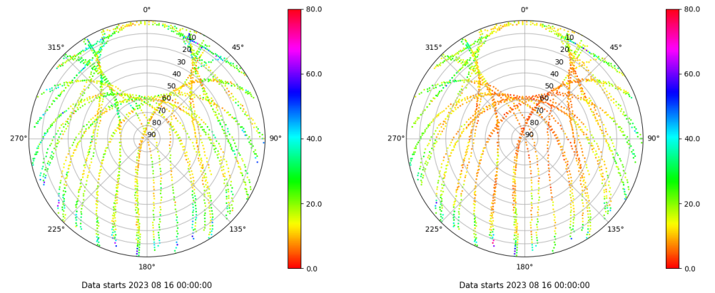
Skyplot for station VALA. Parameter M1C Data file VALA00ESP_R_2023228.xtr Skyplot for station VALA. Parameter M2C Data file VALA00ESP_R_2023228.xtr
