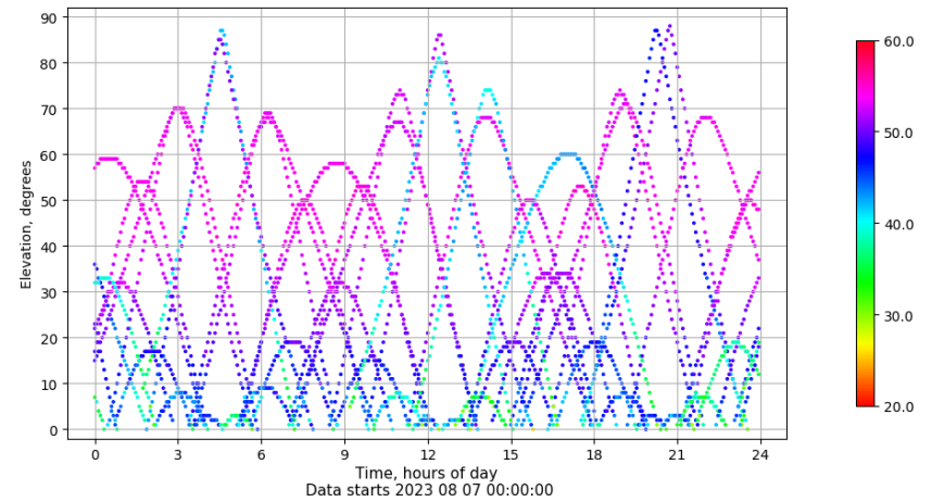
Time-elevation plot for station VALA. Signal to Noise S1C Data file VALA00ESP_R_2023219.xtr
