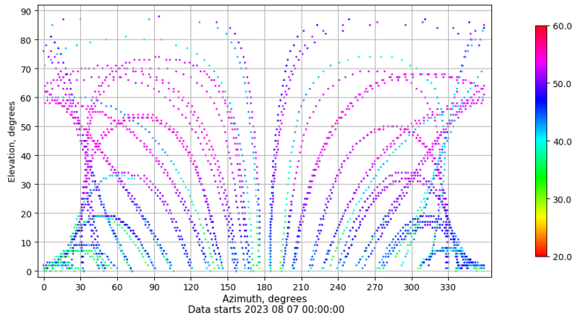
Azimuth-elevation plot for station VALA. Signal to Noise S1C Data file VALA00ESP_R_2023219.xtr
