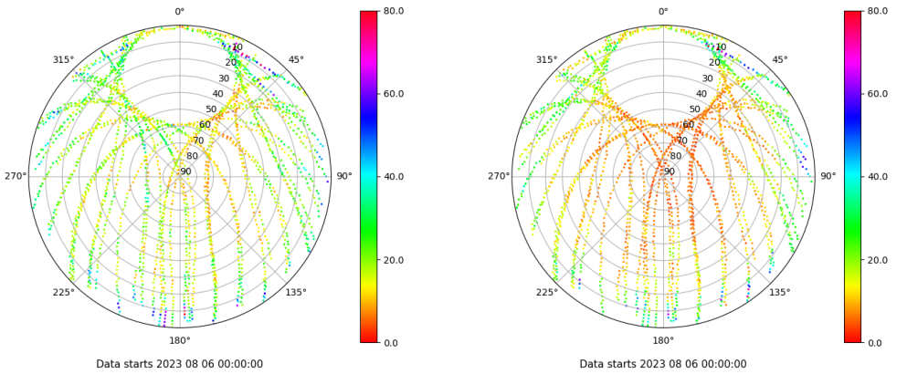
Skyplot for station VALA. Parameter M1C Data file VALA00ESP_R_2023218.xtr Skyplot for station VALA. Parameter M2C Data file VALA00ESP_R_2023218.xtr
