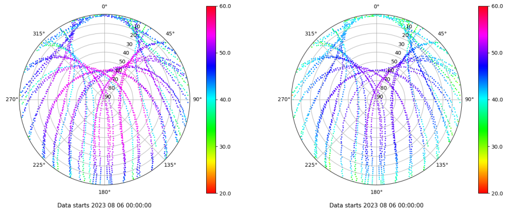
Skyplot for station VALA. Signal to Noise S1C Data file VALA00ESP_R_2023218.xtr Skyplot for station VALA. Signal to Noise S2C Data file VALA00ESP_R_2023218.xtr
