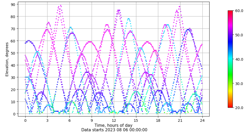
Time-elevation plot for station VALA. Signal to Noise S1C Data file VALA00ESP_R_2023218.xtr
