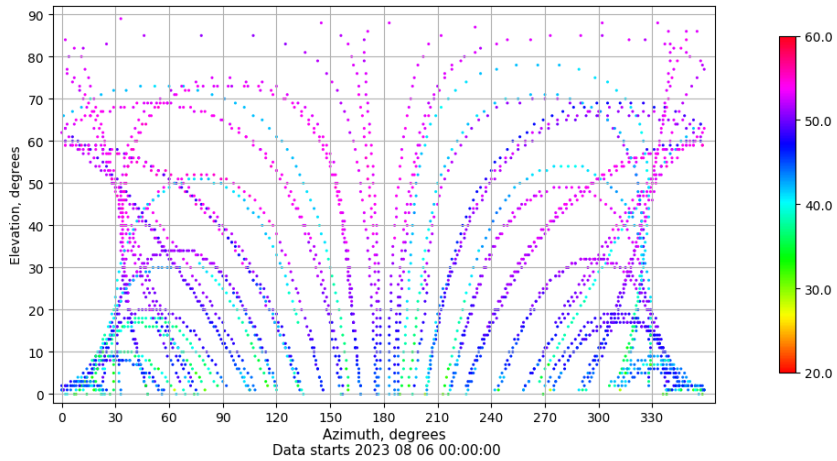
Azimuth-elevation plot for station VALA. Signal to Noise S1C Data file VALA00ESP_R_2023218.xtr
