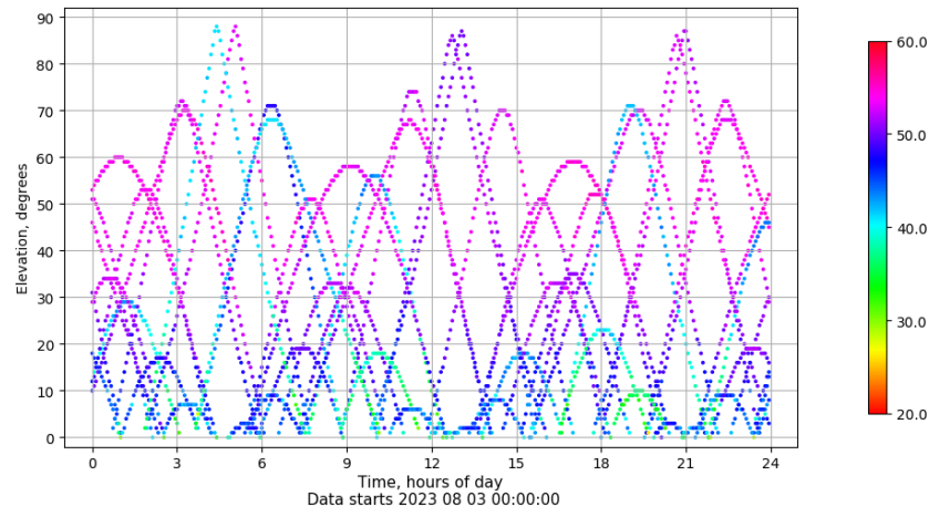
Time-elevation plot for station VALA. Signal to Noise S1C Data file VALA00ESP_R_2023215.xtr
