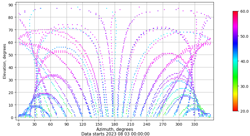
Azimuth-elevation plot for station VALA. Signal to Noise S1C Data file VALA00ESP_R_2023215.xtr
