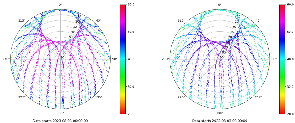
Skyplot for station VALA. Signal to Noise S1C Data file VALA00ESP_R_2023215.xtr Skyplot for station VALA. Signal to Noise S2C Data file VALA00ESP_R_2023215.xtr
