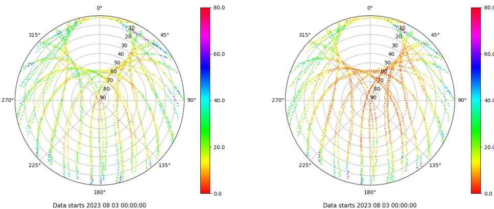
Skyplot for station VALA. Parameter M1C Data file VALA00ESP_R_2023215.xtr Skyplot for station VALA. Parameter M2C Data file VALA00ESP_R_2023215.xtr
