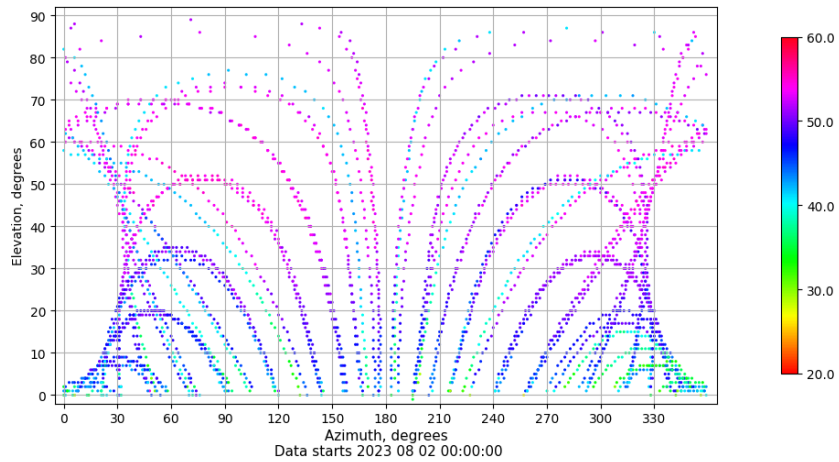
Azimuth-elevation plot for station VALA. Signal to Noise S1C Data file VALA00ESP_R_2023214.xtr
