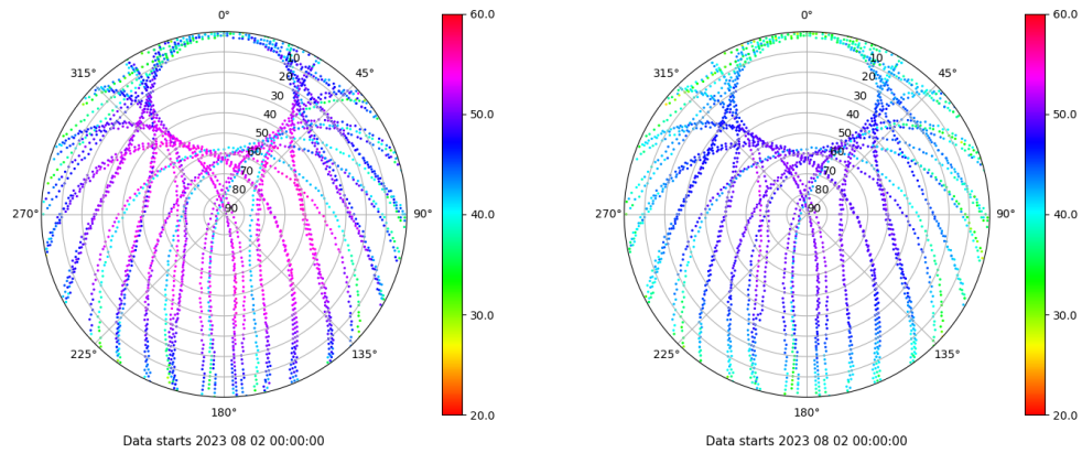
Skyplot for station VALA. Signal to Noise S1C Data file VALA00ESP_R_2023214.xtr Skyplot for station VALA. Signal to Noise S2C Data file VALA00ESP_R_2023214.xtr
