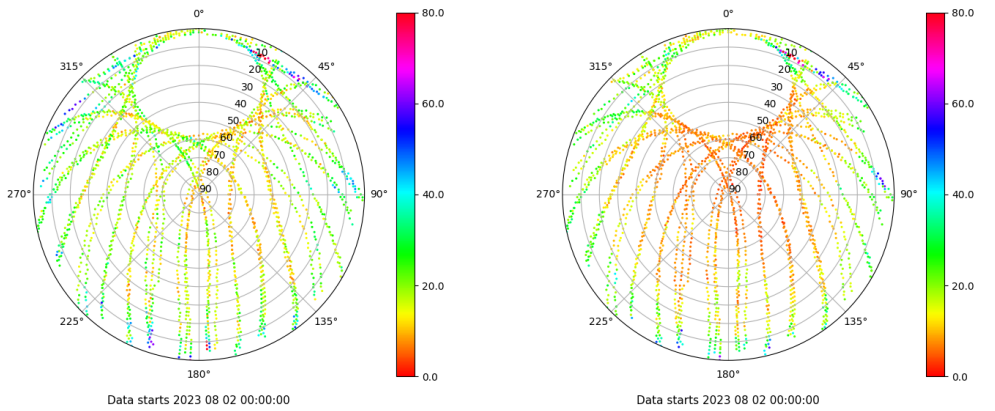
Skyplot for station VALA. Parameter M1C Data file VALA00ESP_R_2023214.xtr Skyplot for station VALA. Parameter M2C Data file VALA00ESP_R_2023214.xtr
