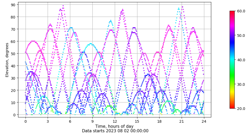
Time-elevation plot for station VALA. Signal to Noise S1C Data file VALA00ESP_R_2023214.xtr
