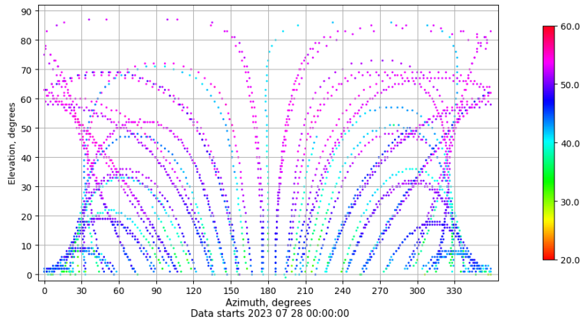
Azimuth-elevation plot for station VALA. Signal to Noise S1C Data file VALA00ESP_R_2023209.xtr
