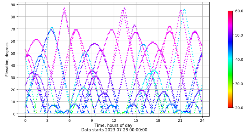
Time-elevation plot for station VALA. Signal to Noise S1C Data file VALA00ESP_R_2023209.xtr
