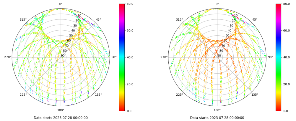
Skyplot for station VALA. Parameter M1C Data file VALA00ESP_R_2023209.xtr Skyplot for station VALA. Parameter M2C Data file VALA00ESP_R_2023209.xtr
