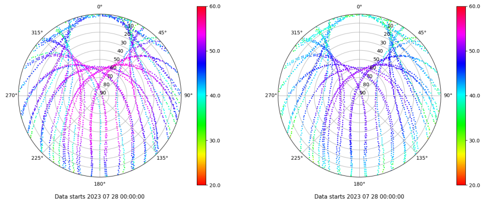
Skyplot for station VALA. Signal to Noise S1C Data file VALA00ESP_R_2023209.xtr Skyplot for station VALA. Signal to Noise S2C Data file VALA00ESP_R_2023209.xtr
