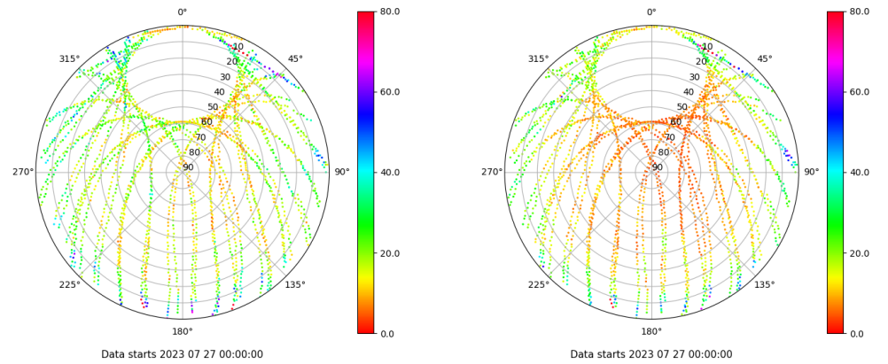
Skyplot for station VALA. Parameter M1C Data file VALA00ESP_R_2023208.xtr Skyplot for station VALA. Parameter M2C Data file VALA00ESP_R_2023208.xtr
