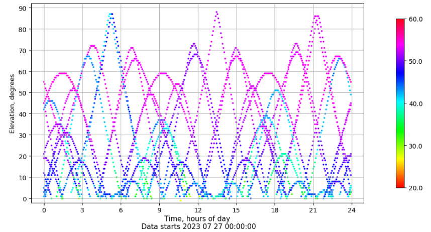
Time-elevation plot for station VALA. Signal to Noise S1C Data file VALA00ESP_R_2023208.xtr
