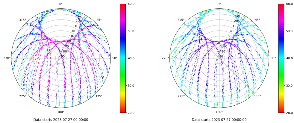
Skyplot for station VALA. Signal to Noise S1C Data file VALA00ESP_R_2023208.xtr Skyplot for station VALA. Signal to Noise S2C Data file VALA00ESP_R_2023208.xtr
