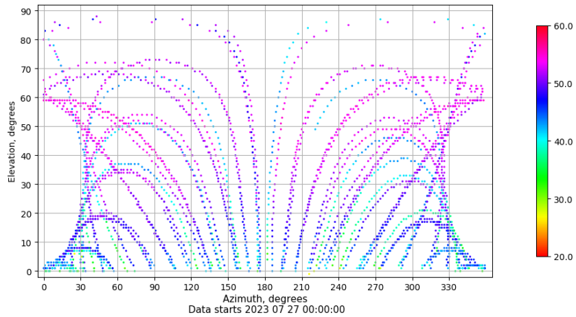
Azimuth-elevation plot for station VALA. Signal to Noise S1C Data file VALA00ESP_R_2023208.xtr
