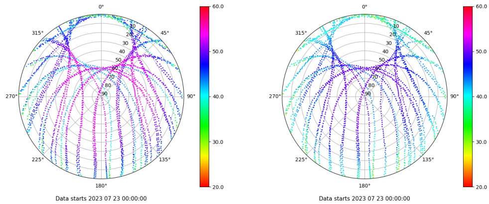
Skyplot for station VALA. Signal to Noise S1C Data file VALA00ESP_R_2023204.xtr Skyplot for station VALA. Signal to Noise S2C Data file VALA00ESP_R_2023204.xtr
