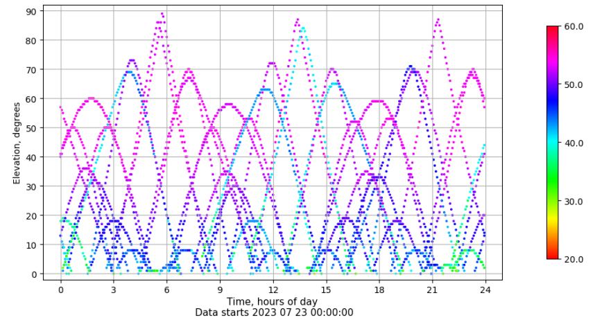
Time-elevation plot for station VALA. Signal to Noise S1C Data file VALA00ESP_R_2023204.xtr
