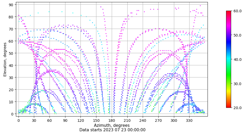
Azimuth-elevation plot for station VALA. Signal to Noise S1C Data file VALA00ESP_R_2023204.xtr
