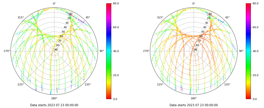
Skyplot for station VALA. Parameter M1C Data file VALA00ESP_R_2023204.xtr Skyplot for station VALA. Parameter M2C Data file VALA00ESP_R_2023204.xtr
