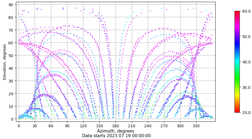
Azimuth-elevation plot for station VALA. Signal to Noise S1C Data file VALA00ESP_R_2023200.xtr
