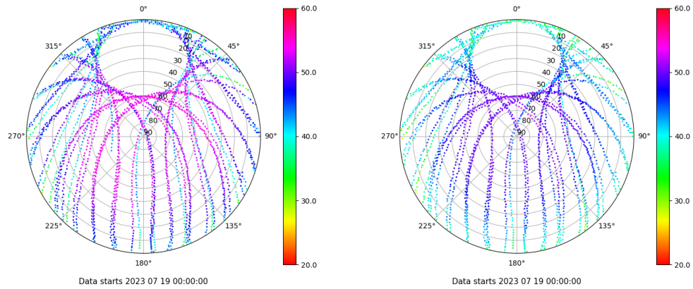
Skyplot for station VALA. Signal to Noise S1C Data file VALA00ESP_R_2023200.xtr Skyplot for station VALA. Signal to Noise S2C Data file VALA00ESP_R_2023200.xtr
