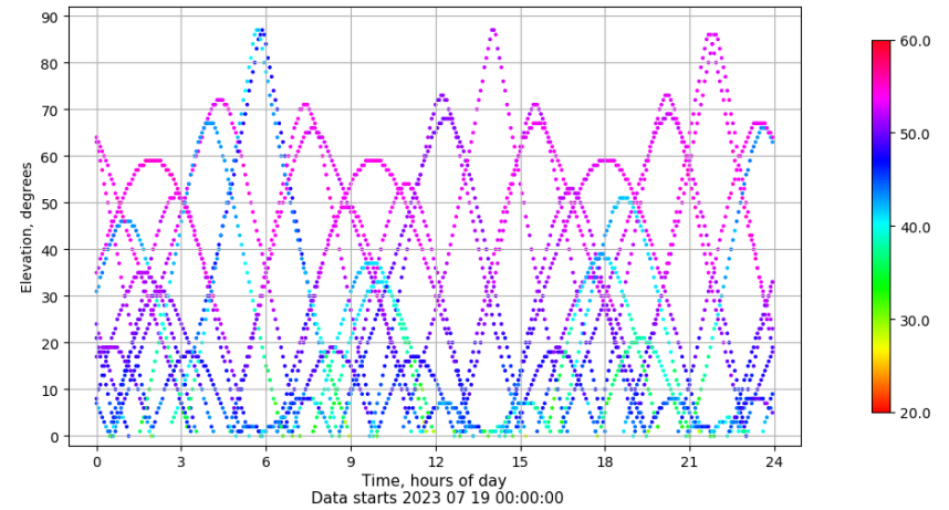
Time-elevation plot for station VALA. Signal to Noise S1C Data file VALA00ESP_R_2023200.xtr
