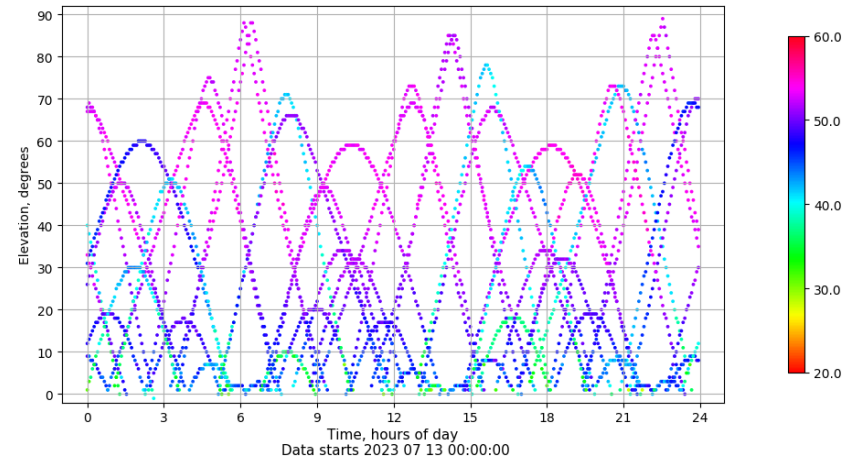
Time-elevation plot for station VALA. Signal to Noise S1C Data file VALA00ESP_R_2023194.xtr
