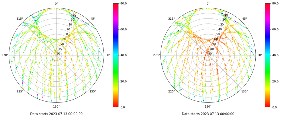
Skyplot for station VALA. Parameter M1C Data file VALA00ESP_R_2023194.xtr Skyplot for station VALA. Parameter M2C Data file VALA00ESP_R_2023194.xtr
