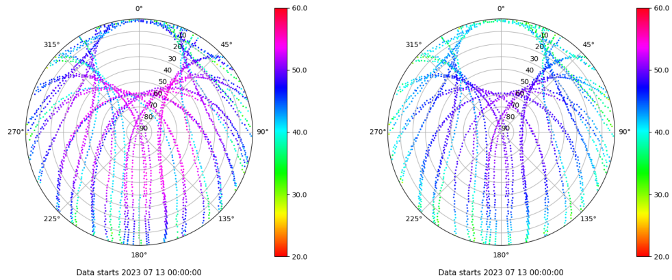
Skyplot for station VALA. Signal to Noise S1C Data file VALA00ESP_R_2023194.xtr Skyplot for station VALA. Signal to Noise S2C Data file VALA00ESP_R_2023194.xtr
