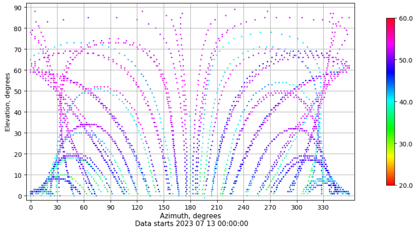
Azimuth-elevation plot for station VALA. Signal to Noise S1C Data file VALA00ESP_R_2023194.xtr
