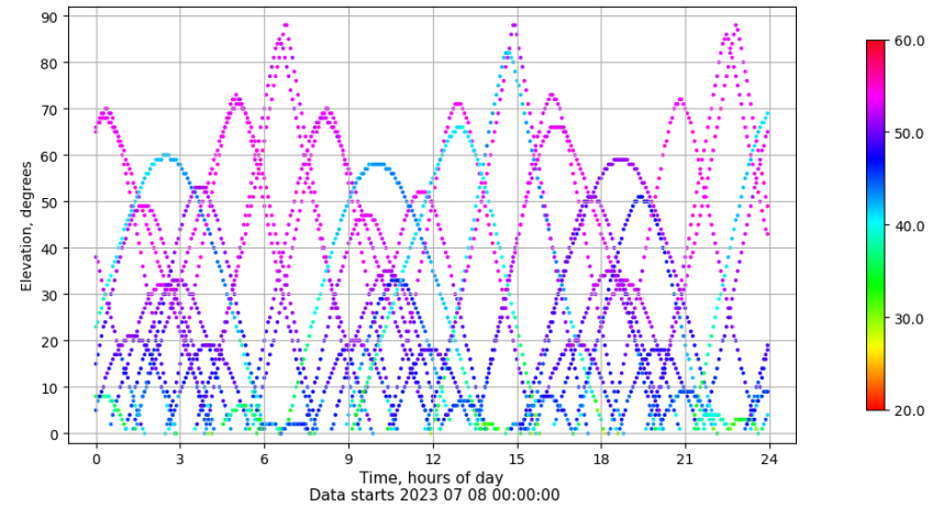
Time-elevation plot for station VALA. Signal to Noise S1C Data file VALA00ESP_R_2023189.xtr
