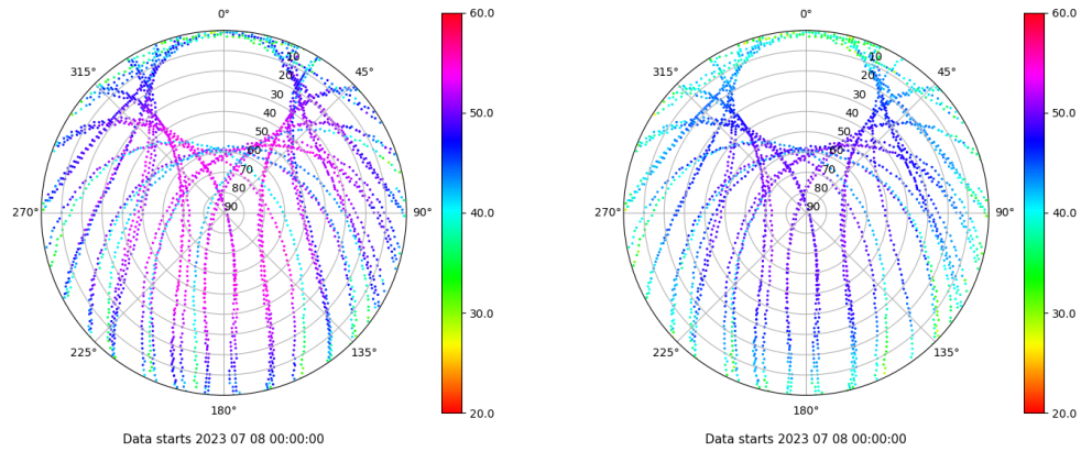
Skyplot for station VALA. Signal to Noise S1C Data file VALA00ESP_R_2023189.xtr Skyplot for station VALA. Signal to Noise S2C Data file VALA00ESP_R_2023189.xtr
