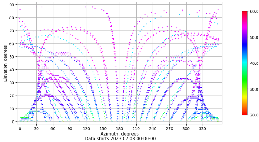
Azimuth-elevation plot for station VALA. Signal to Noise S1C Data file VALA00ESP_R_2023189.xtr
