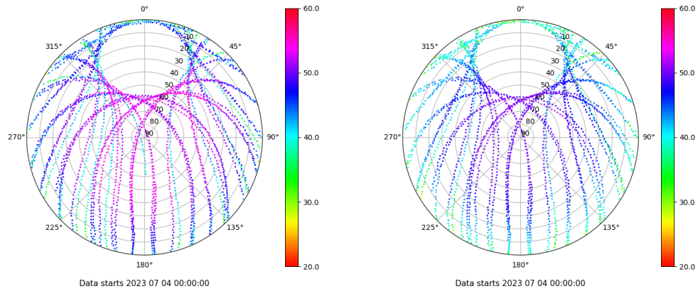
Skyplot for station VALA. Signal to Noise S1C Data file VALA00ESP_R_2023185.xtr Skyplot for station VALA. Signal to Noise S2C Data file VALA00ESP_R_2023185.xtr
