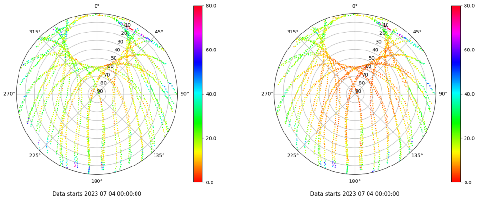
Skyplot for station VALA. Parameter M1C Data file VALA00ESP_R_2023185.xtr Skyplot for station VALA. Parameter M2C Data file VALA00ESP_R_2023185.xtr
