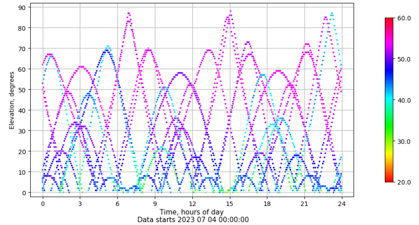
Time-elevation plot for station VALA. Signal to Noise S1C Data file VALA00ESP_R_2023185.xtr
