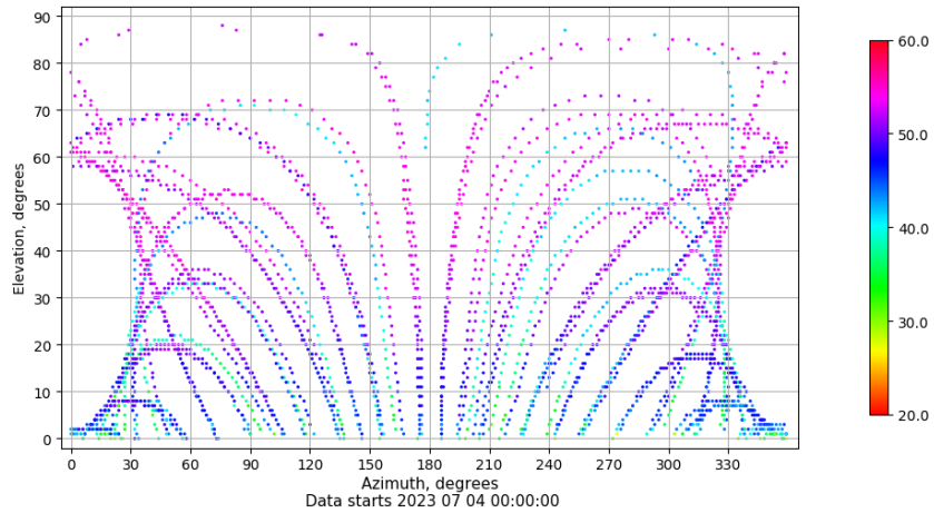
Azimuth-elevation plot for station VALA. Signal to Noise S1C Data file VALA00ESP_R_2023185.xtr
