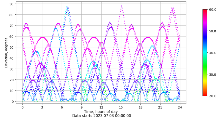
Time-elevation plot for station VALA. Signal to Noise S1C Data file VALA00ESP_R_2023184.xtr
