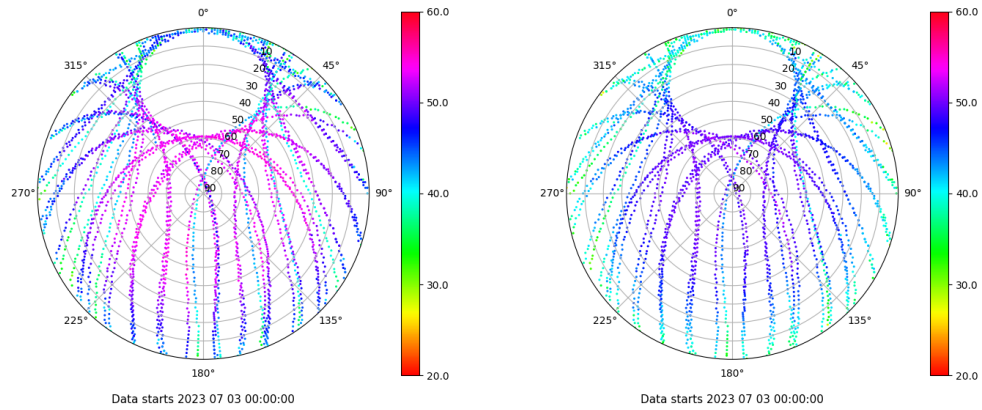
Skyplot for station VALA. Signal to Noise S1C Data file VALA00ESP_R_2023184.xtr Skyplot for station VALA. Signal to Noise S2C Data file VALA00ESP_R_2023184.xtr
