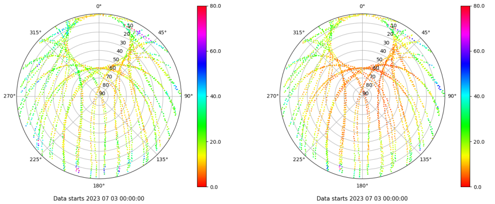
Skyplot for station VALA. Parameter M1C Data file VALA00ESP_R_2023184.xtr Skyplot for station VALA. Parameter M2C Data file VALA00ESP_R_2023184.xtr
