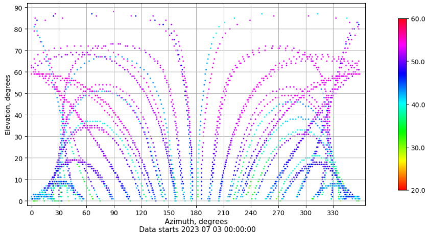
Azimuth-elevation plot for station VALA. Signal to Noise S1C Data file VALA00ESP_R_2023184.xtr
