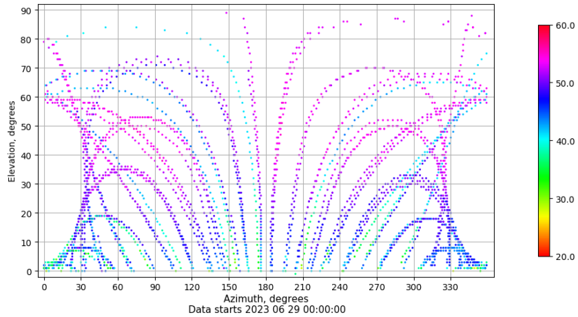
Azimuth-elevation plot for station VALA. Signal to Noise S1C Data file VALA00ESP_R_2023180.xtr
