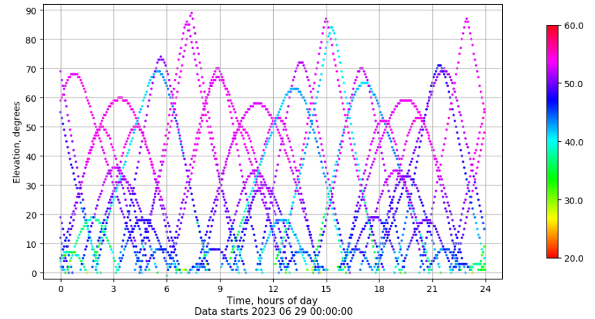
Time-elevation plot for station VALA. Signal to Noise S1C Data file VALA00ESP_R_2023180.xtr
