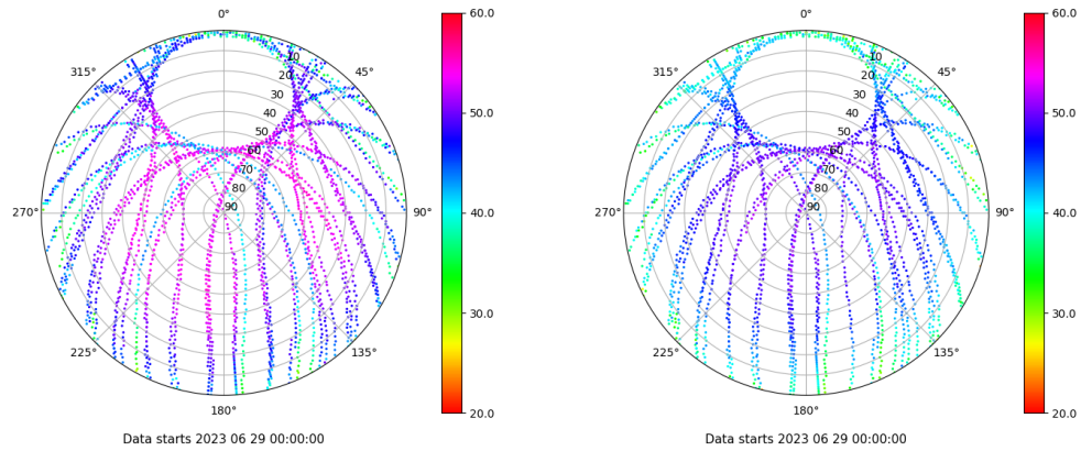
Skyplot for station VALA. Signal to Noise S1C Data file VALA00ESP_R_2023180.xtr Skyplot for station VALA. Signal to Noise S2C Data file VALA00ESP_R_2023180.xtr
