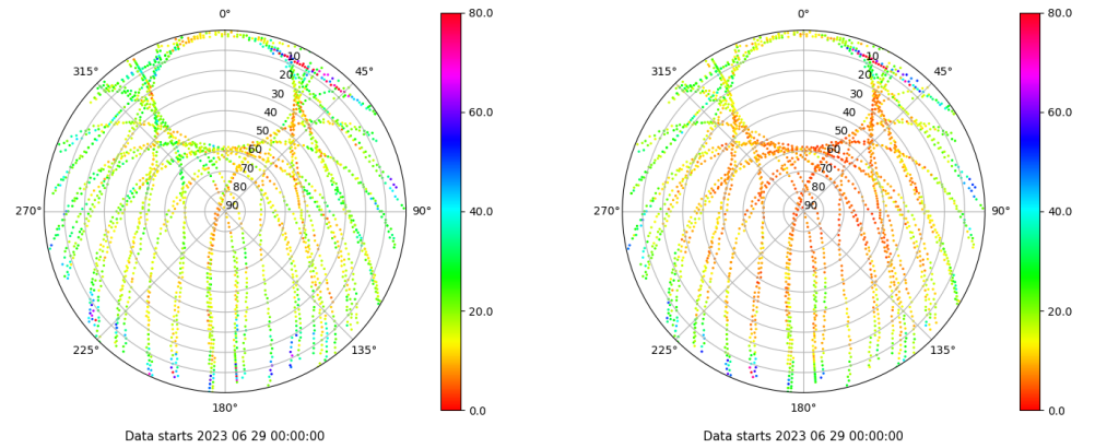
Skyplot for station VALA. Parameter M1C Data file VALA00ESP_R_2023180.xtr Skyplot for station VALA. Parameter M2C Data file VALA00ESP_R_2023180.xtr
