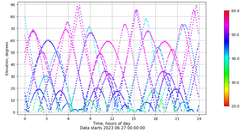
Time-elevation plot for station VALA. Signal to Noise S1C Data file VALA00ESP_R_2023178.xtr
