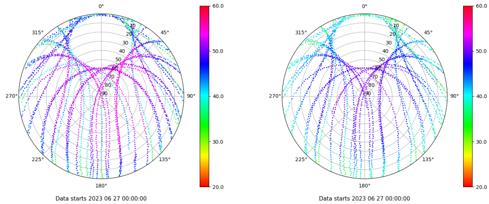
Skyplot for station VALA. Signal to Noise S1C Data file VALA00ESP_R_2023178.xtr Skyplot for station VALA. Signal to Noise S2C Data file VALA00ESP_R_2023178.xtr
