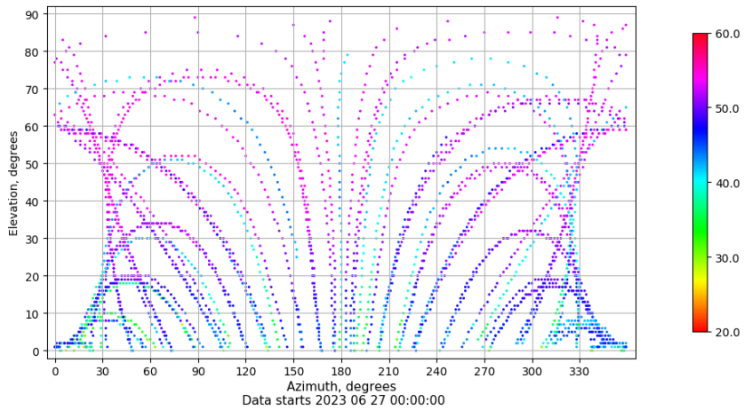
Azimuth-elevation plot for station VALA. Signal to Noise S1C Data file VALA00ESP_R_2023178.xtr
