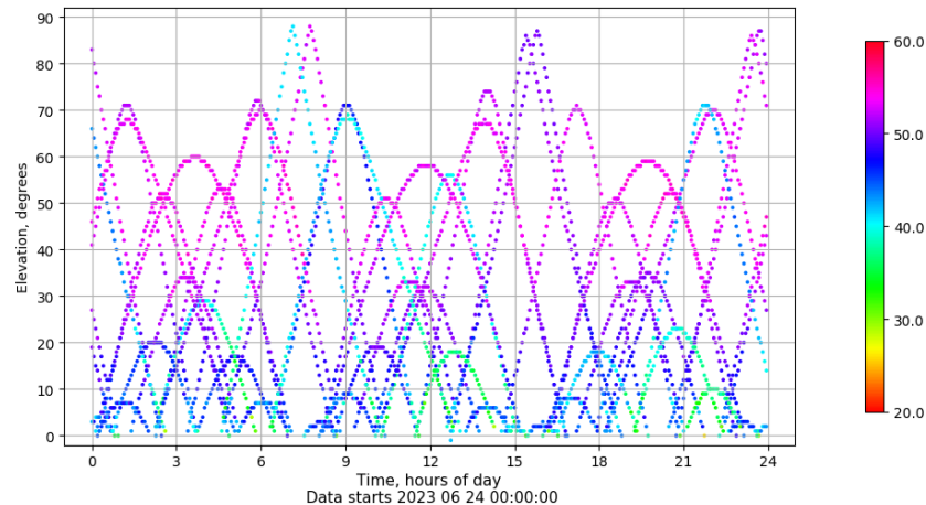
Time-elevation plot for station VALA. Signal to Noise S1C Data file VALA00ESP_R_2023175.xtr
