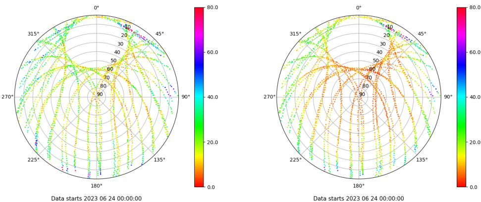
Skyplot for station VALA. Parameter M1C Data file VALA00ESP_R_2023175.xtr Skyplot for station VALA. Parameter M2C Data file VALA00ESP_R_2023175.xtr
