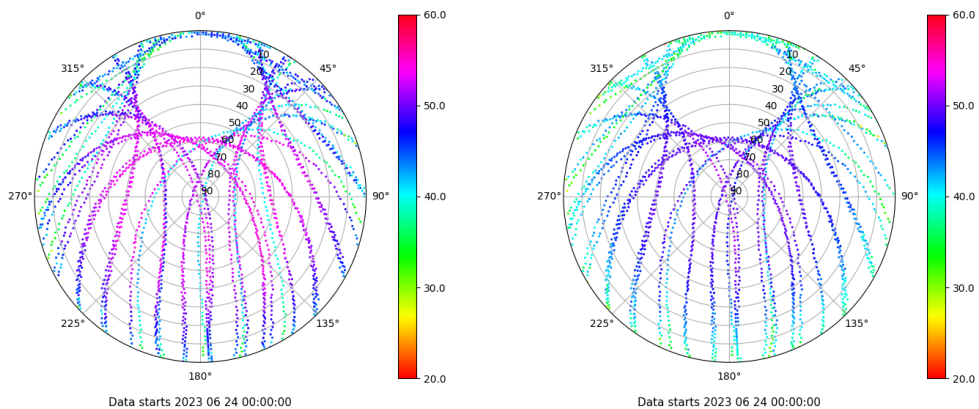
Skyplot for station VALA. Signal to Noise S1C Data file VALA00ESP_R_2023175.xtr Skyplot for station VALA. Signal to Noise S2C Data file VALA00ESP_R_2023175.xtr
