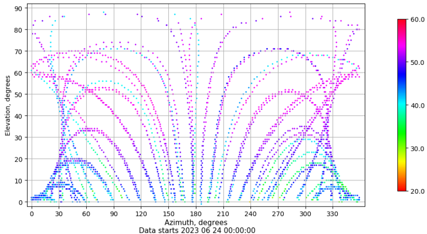
Azimuth-elevation plot for station VALA. Signal to Noise S1C Data file VALA00ESP_R_2023175.xtr
