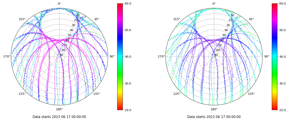
Skyplot for station VALA. Signal to Noise S1C Data file VALA00ESP_R_2023168.xtr Skyplot for station VALA. Signal to Noise S2C Data file VALA00ESP_R_2023168.xtr
