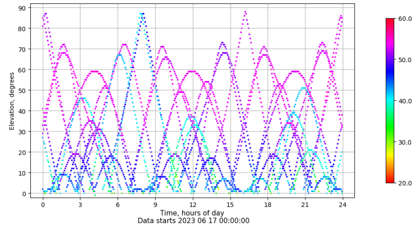
Time-elevation plot for station VALA. Signal to Noise S1C Data file VALA00ESP_R_2023168.xtr
