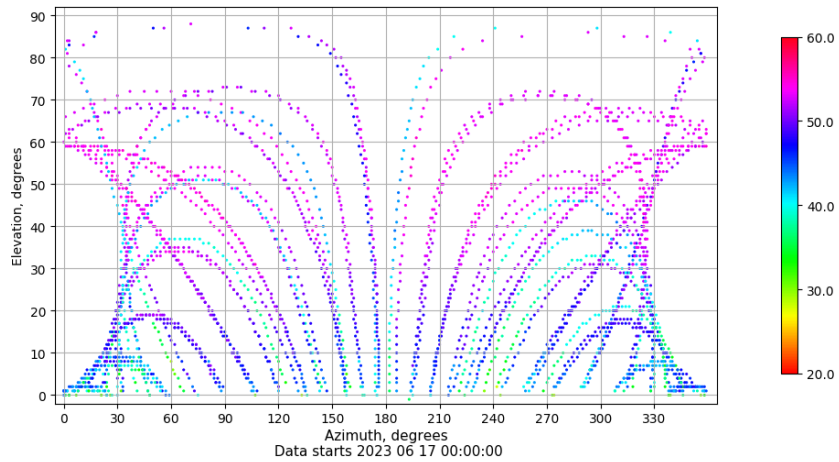
Azimuth-elevation plot for station VALA. Signal to Noise S1C Data file VALA00ESP_R_2023168.xtr
