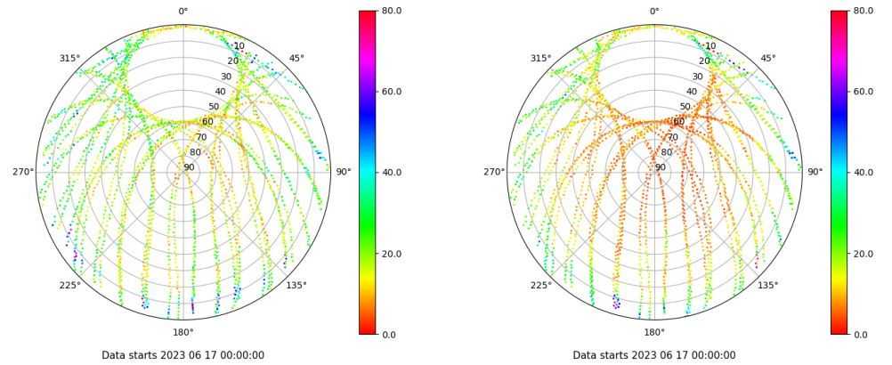
Skyplot for station VALA. Parameter M1C Data file VALA00ESP_R_2023168.xtr Skyplot for station VALA. Parameter M2C Data file VALA00ESP_R_2023168.xtr
