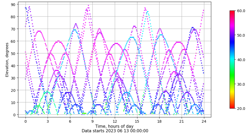
Time-elevation plot for station VALA. Signal to Noise S1C Data file VALA00ESP_R_2023164.xtr
