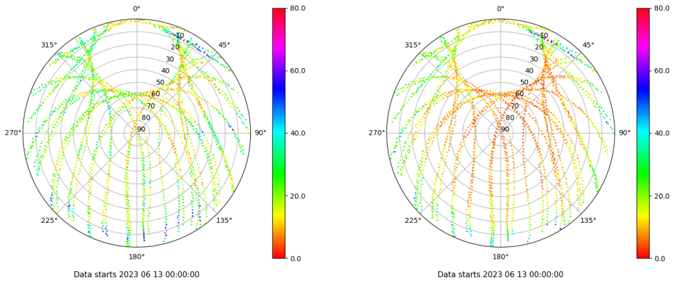
Skyplot for station VALA. Parameter M1C Data file VALA00ESP_R_2023164.xtr Skyplot for station VALA. Parameter M2C Data file VALA00ESP_R_2023164.xtr
