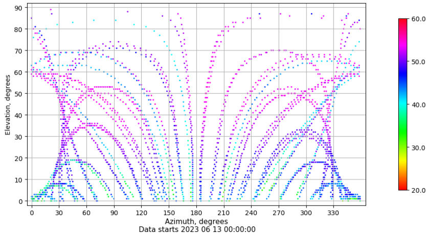
Azimuth-elevation plot for station VALA. Signal to Noise S1C Data file VALA00ESP_R_2023164.xtr
