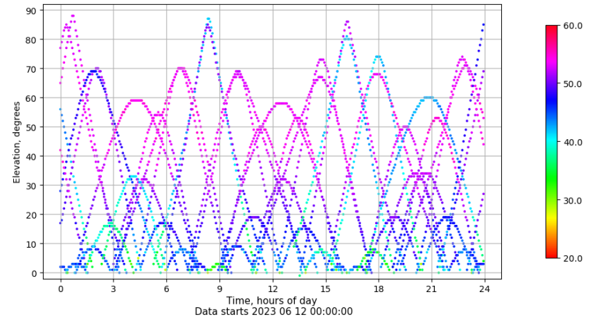
Time-elevation plot for station VALA. Signal to Noise S1C Data file VALA00ESP_R_2023163.xtr
