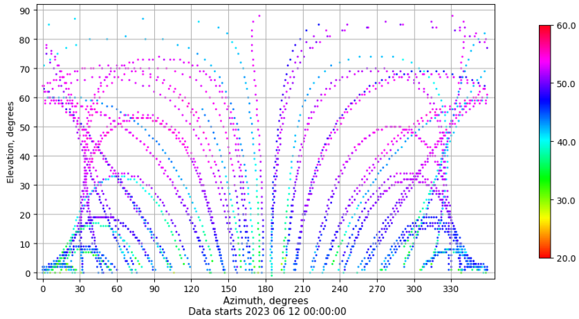
Azimuth-elevation plot for station VALA. Signal to Noise S1C Data file VALA00ESP_R_2023163.xtr
