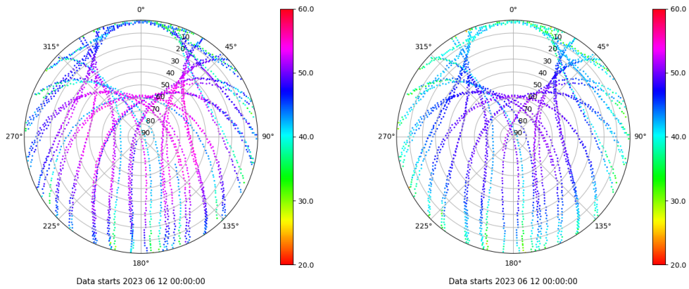
Skyplot for station VALA. Signal to Noise S1C Data file VALA00ESP_R_2023163.xtr Skyplot for station VALA. Signal to Noise S2C Data file VALA00ESP_R_2023163.xtr
