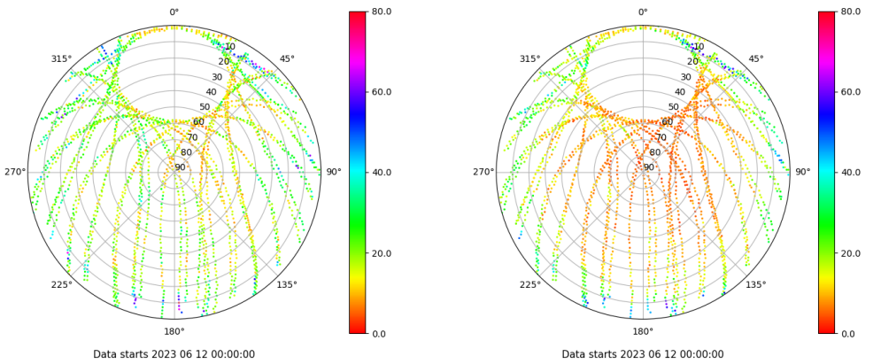
Skyplot for station VALA. Parameter M1C Data file VALA00ESP_R_2023163.xtr Skyplot for station VALA. Parameter M2C Data file VALA00ESP_R_2023163.xtr
