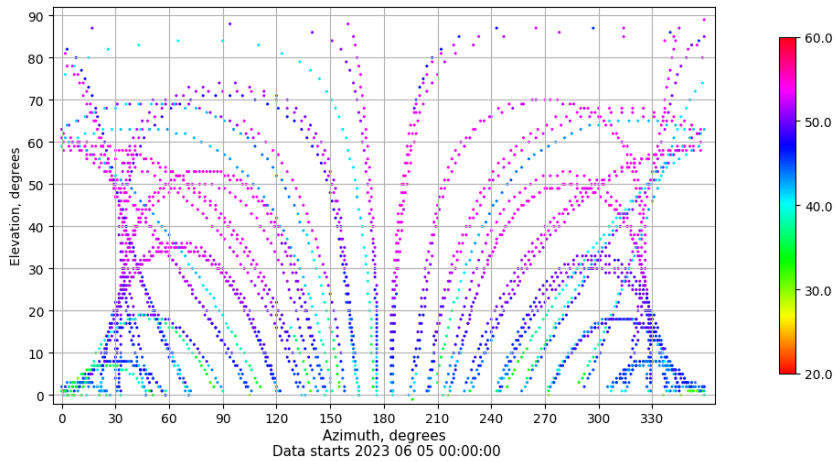
Azimuth-elevation plot for station VALA. Signal to Noise S1C Data file VALA00ESP_R_2023156.xtr
