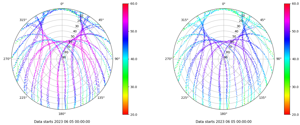
Skyplot for station VALA. Signal to Noise S1C Data file VALA00ESP_R_2023156.xtr Skyplot for station VALA. Signal to Noise S2C Data file VALA00ESP_R_2023156.xtr
