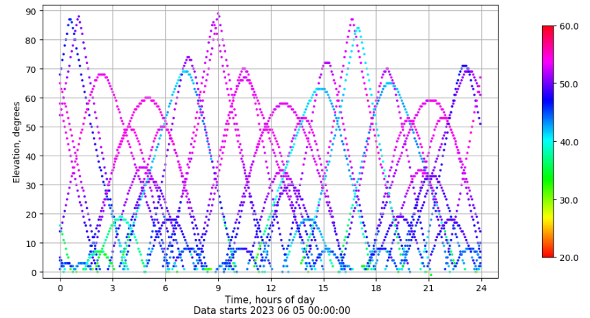
Time-elevation plot for station VALA. Signal to Noise S1C Data file VALA00ESP_R_2023156.xtr
