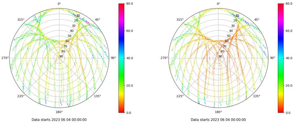
Skyplot for station VALA. Parameter M1C Data file VALA00ESP_R_2023155.xtr Skyplot for station VALA. Parameter M2C Data file VALA00ESP_R_2023155.xtr
