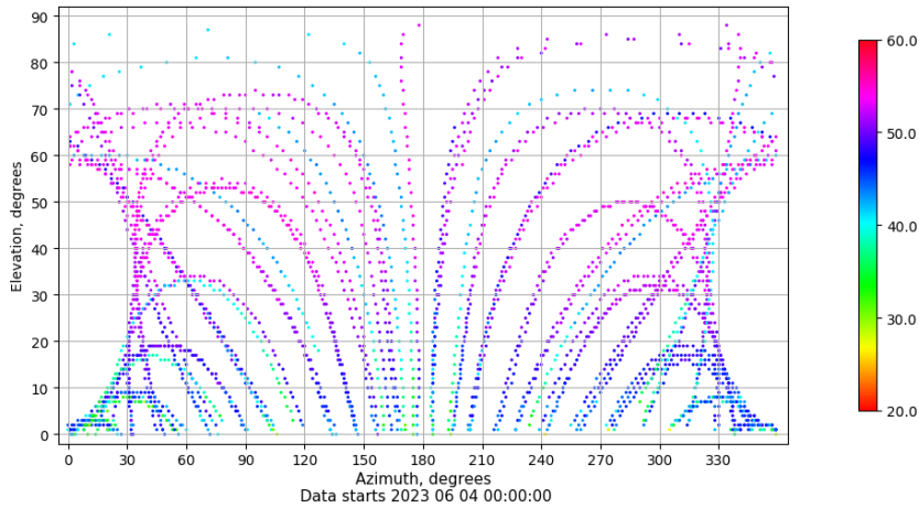
Azimuth-elevation plot for station VALA. Signal to Noise S1C Data file VALA00ESP_R_2023155.xtr
