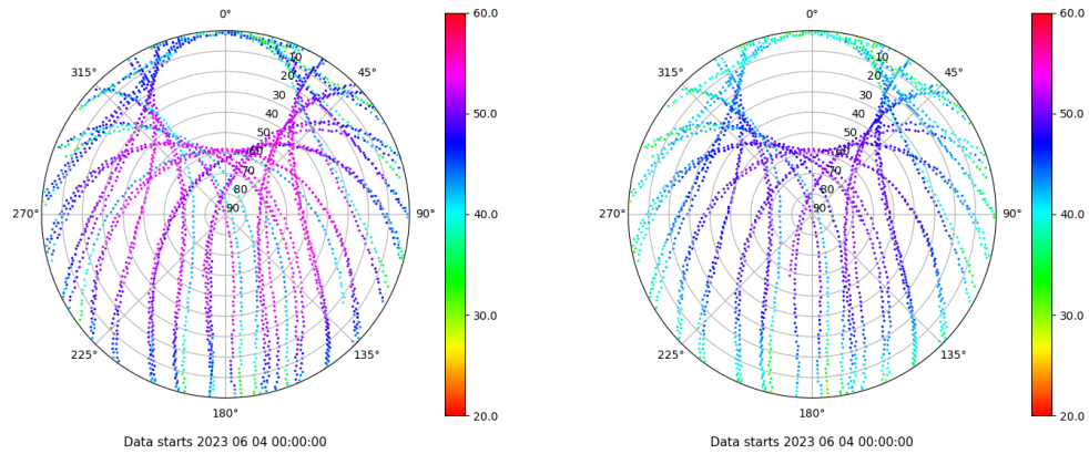
Skyplot for station VALA. Signal to Noise S1C Data file VALA00ESP_R_2023155.xtr Skyplot for station VALA. Signal to Noise S2C Data file VALA00ESP_R_2023155.xtr
