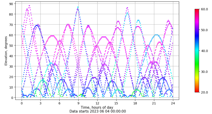
Time-elevation plot for station VALA. Signal to Noise S1C Data file VALA00ESP_R_2023155.xtr
