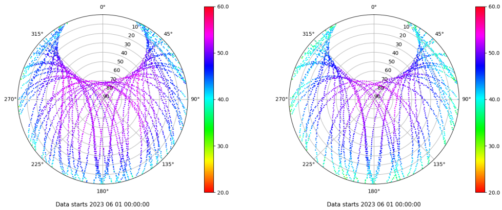
Skyplot for station VALA. Signal to Noise S1C Data file VALA00ESP_R_2023152.xtr Skyplot for station VALA. Signal to Noise S2S Data file VALA00ESP_R_2023152.xtr
