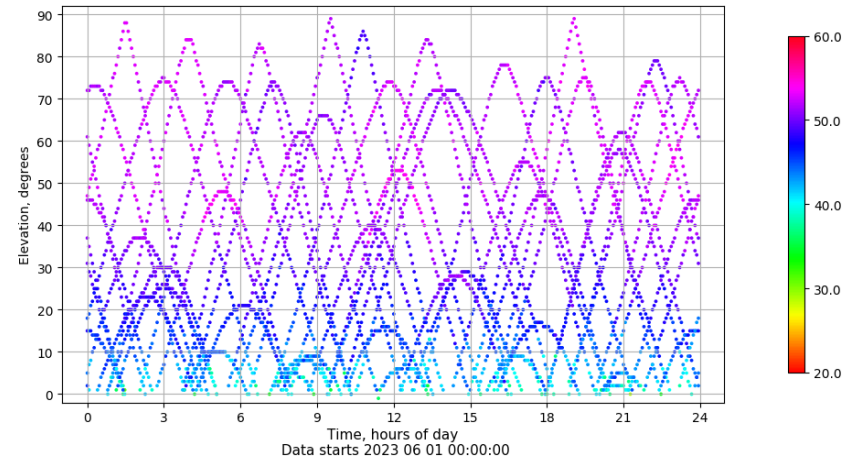
Time-elevation plot for station VALA. Signal to Noise S1C Data file VALA00ESP_R_2023152.xtr
