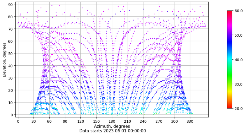
Azimuth-elevation plot for station VALA. Signal to Noise S1C Data file VALA00ESP_R_2023152.xtr
