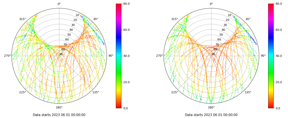
Skyplot for station VALA. Parameter M1C Data file VALA00ESP_R_2023152.xtr Skyplot for station VALA. Parameter M2S Data file VALA00ESP_R_2023152.xtr
