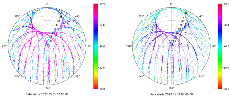
Skyplot for station VALA. Signal to Noise S1C Data file VALA00ESP_R_2023151.xtr Skyplot for station VALA. Signal to Noise S2C Data file VALA00ESP_R_2023151.xtr
