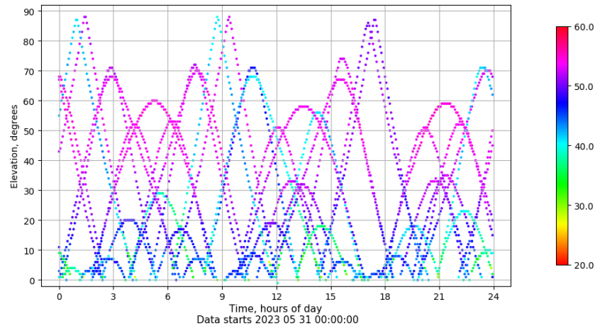
Time-elevation plot for station VALA. Signal to Noise S1C Data file VALA00ESP_R_2023151.xtr
