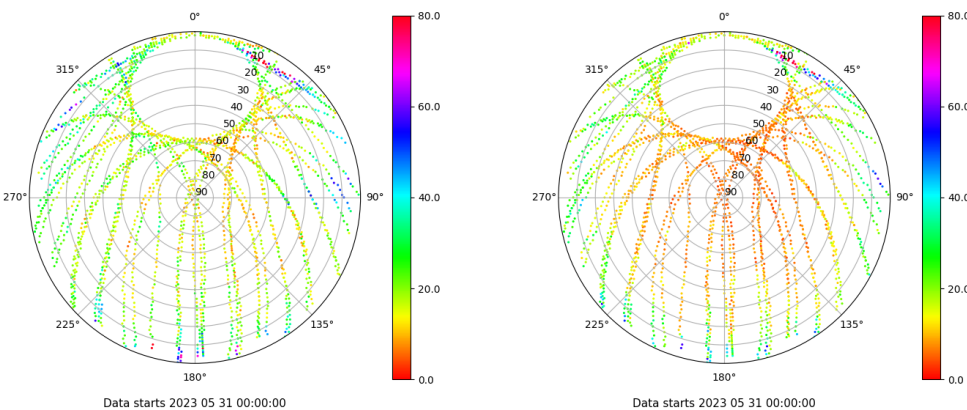
Skyplot for station VALA. Parameter M1C Data file VALA00ESP_R_2023151.xtr Skyplot for station VALA. Parameter M2C Data file VALA00ESP_R_2023151.xtr
