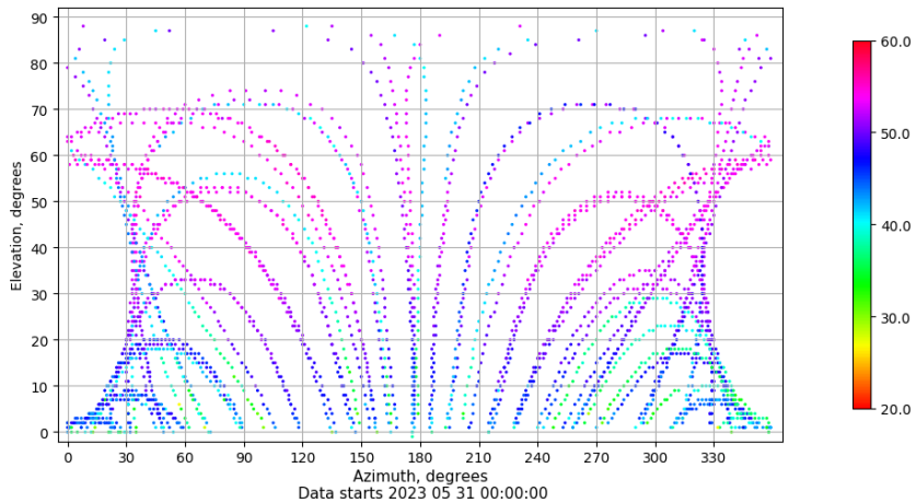
Azimuth-elevation plot for station VALA. Signal to Noise S1C Data file VALA00ESP_R_2023151.xtr
