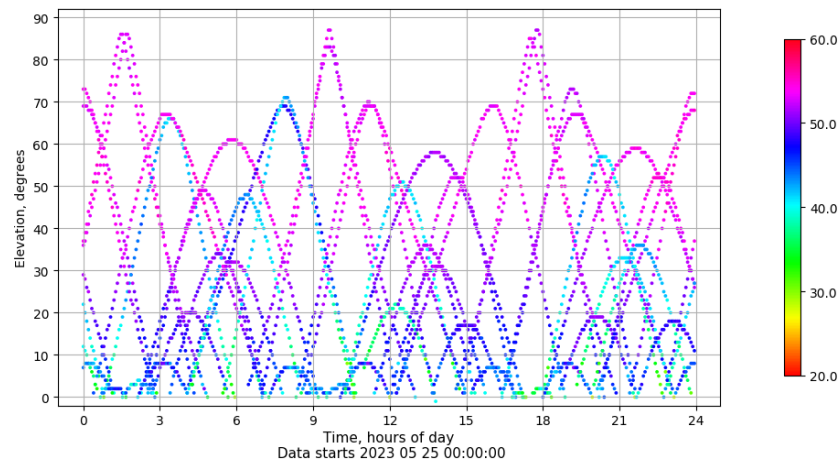
Time-elevation plot for station VALA. Signal to Noise S1C Data file VALA00ESP_R_2023145.xtr
