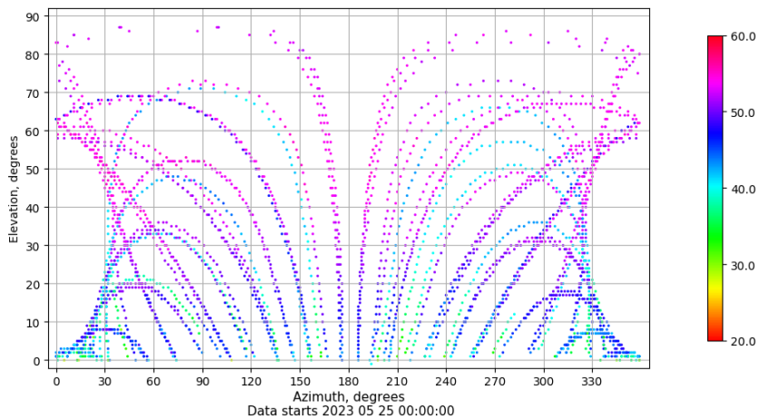
Azimuth-elevation plot for station VALA. Signal to Noise S1C Data file VALA00ESP_R_2023145.xtr
