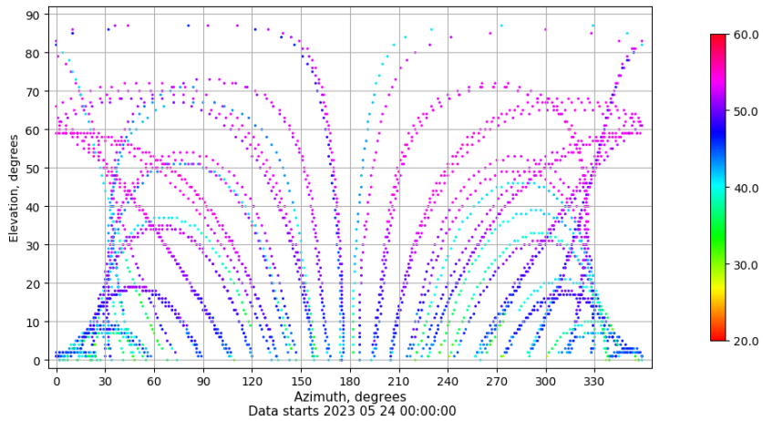
Azimuth-elevation plot for station VALA. Signal to Noise S1C Data file VALA00ESP_R_2023144.xtr
