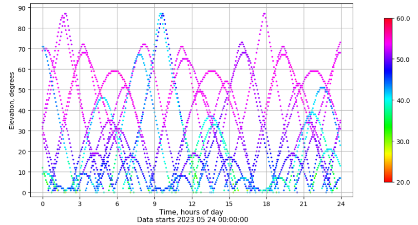
Time-elevation plot for station VALA. Signal to Noise S1C Data file VALA00ESP_R_2023144.xtr
