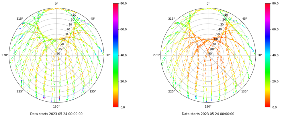
Skyplot for station VALA. Parameter M1C Data file VALA00ESP_R_2023144.xtr Skyplot for station VALA. Parameter M2C Data file VALA00ESP_R_2023144.xtr
