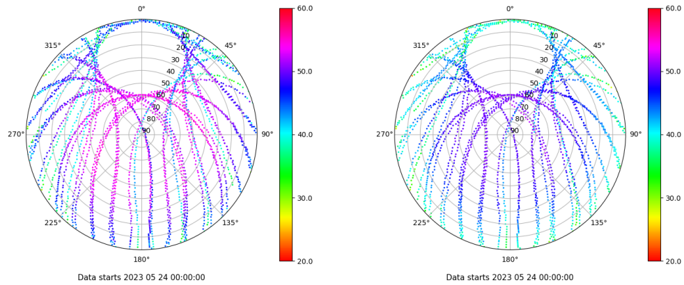
Skyplot for station VALA. Signal to Noise S1C Data file VALA00ESP_R_2023144.xtr Skyplot for station VALA. Signal to Noise S2C Data file VALA00ESP_R_2023144.xtr
