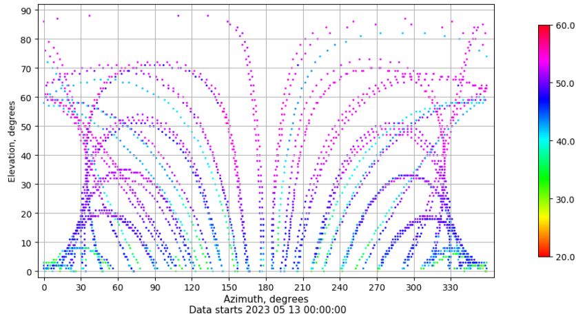
Azimuth-elevation plot for station VALA. Signal to Noise S1C Data file VALA00ESP_R_2023133.xtr
