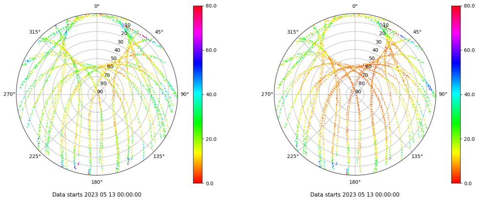
Skyplot for station VALA. Parameter M1C Data file VALA00ESP_R_2023133.xtr Skyplot for station VALA. Parameter M2C Data file VALA00ESP_R_2023133.xtr
