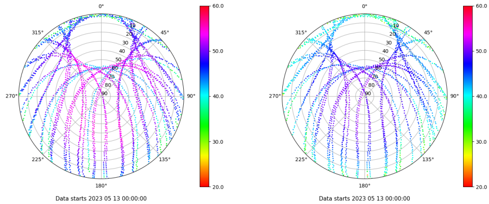
Skyplot for station VALA. Signal to Noise S1C Data file VALA00ESP_R_2023133.xtr Skyplot for station VALA. Signal to Noise S2C Data file VALA00ESP_R_2023133.xtr
