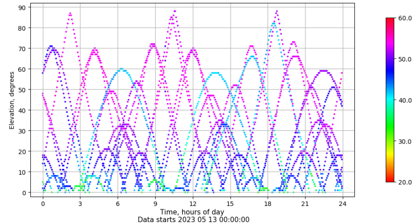
Time-elevation plot for station VALA. Signal to Noise S1C Data file VALA00ESP_R_2023133.xtr
