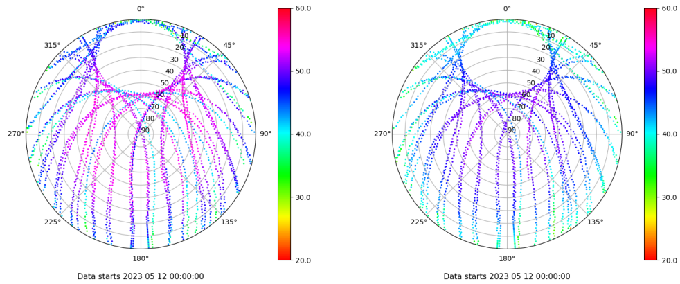
Skyplot for station VALA. Signal to Noise S1C Data file VALA00ESP_R_2023132.xtr Skyplot for station VALA. Signal to Noise S2C Data file VALA00ESP_R_2023132.xtr
