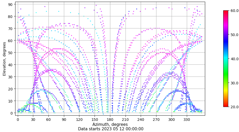
Azimuth-elevation plot for station VALA. Signal to Noise S1C Data file VALA00ESP_R_2023132.xtr
