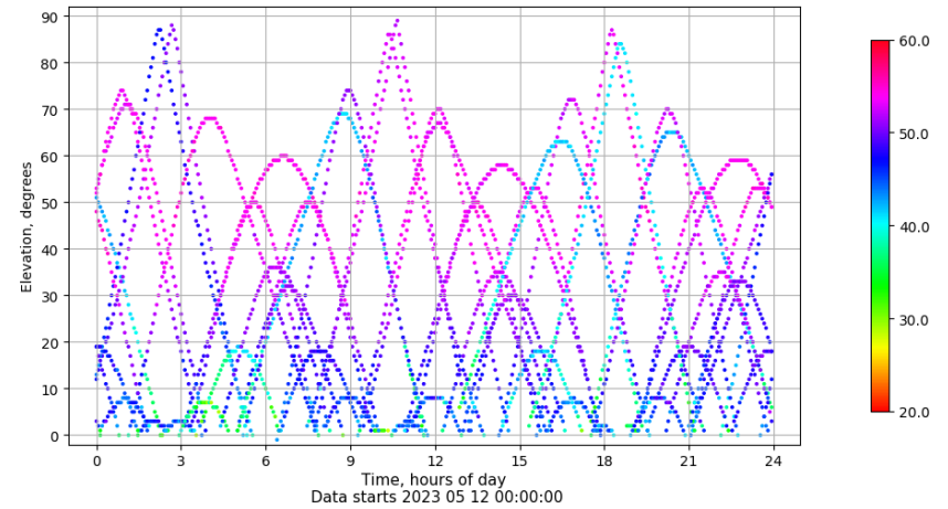
Time-elevation plot for station VALA. Signal to Noise S1C Data file VALA00ESP_R_2023132.xtr
