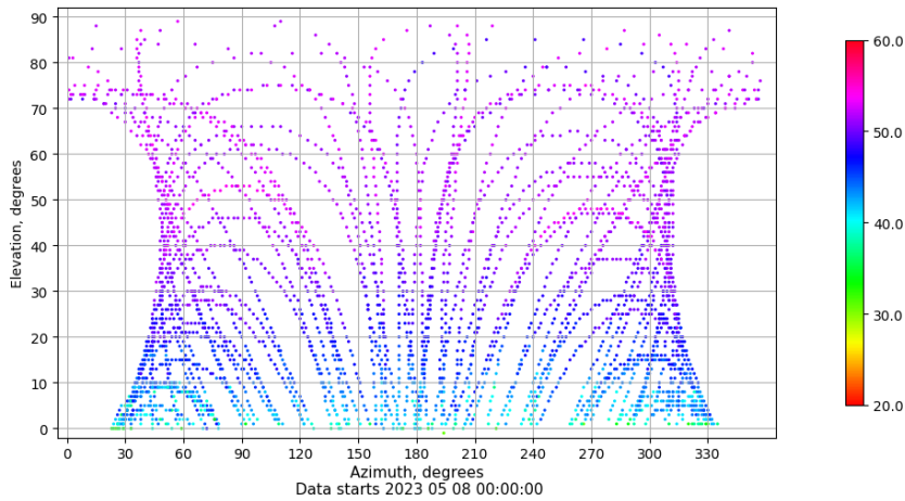
Azimuth-elevation plot for station VALA. Signal to Noise S1C Data file VALA00ESP_R_2023128.xtr
