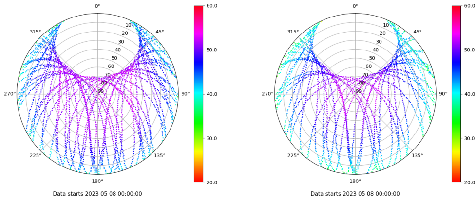
Skyplot for station VALA. Signal to Noise S1C Data file VALA00ESP_R_2023128.xtr Skyplot for station VALA. Signal to Noise S2S Data file VALA00ESP_R_2023128.xtr
