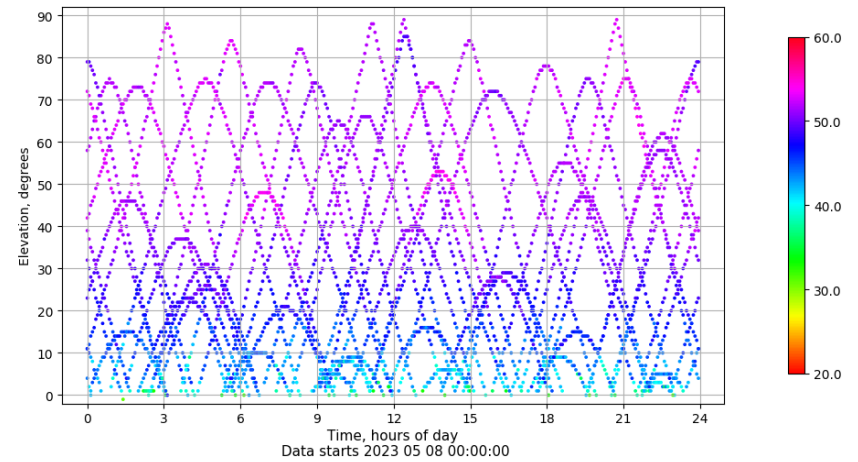
Time-elevation plot for station VALA. Signal to Noise S1C Data file VALA00ESP_R_2023128.xtr
