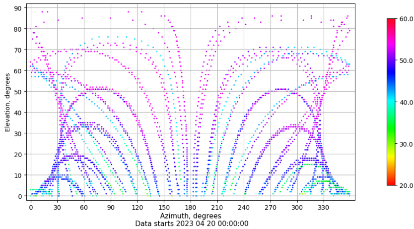
Azimuth-elevation plot for station VALA. Signal to Noise S1C Data file VALA00ESP_R_2023110.xtr
