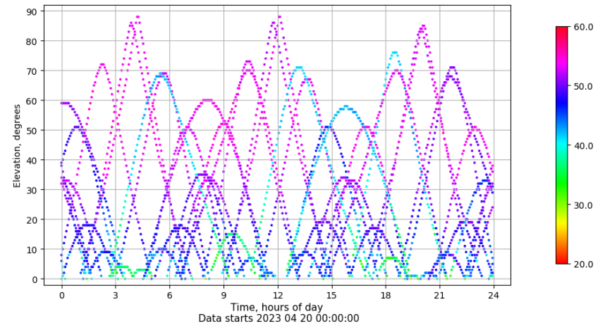
Time-elevation plot for station VALA. Signal to Noise S1C Data file VALA00ESP_R_2023110.xtr
