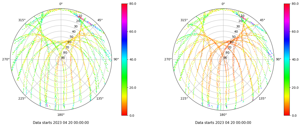
Skyplot for station VALA. Parameter M1C Data file VALA00ESP_R_2023110.xtr Skyplot for station VALA. Parameter M2C Data file VALA00ESP_R_2023110.xtr
