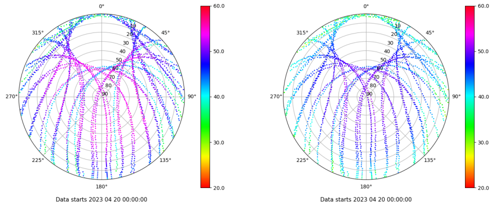
Skyplot for station VALA. Signal to Noise S1C Data file VALA00ESP_R_2023110.xtr Skyplot for station VALA. Signal to Noise S2C Data file VALA00ESP_R_2023110.xtr
