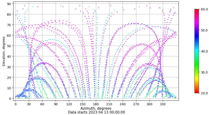
Azimuth-elevation plot for station VALA. Signal to Noise S1C Data file VALA00ESP_R_2023103.xtr
