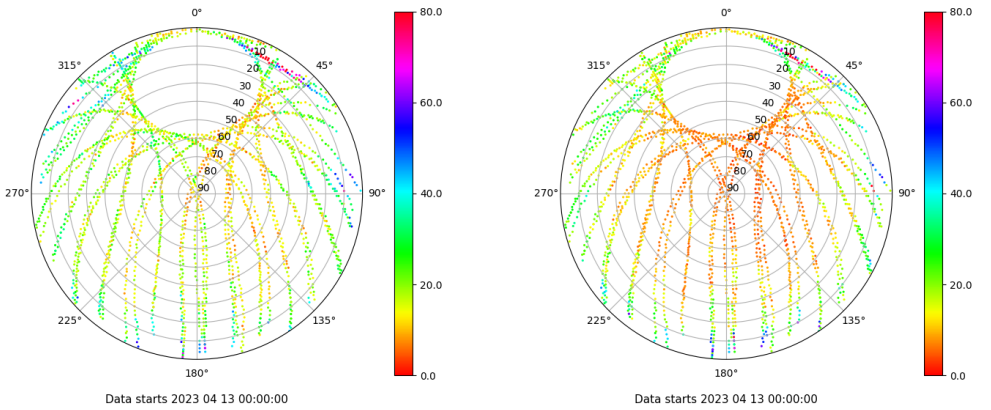
Skyplot for station VALA. Parameter M1C Data file VALA00ESP_R_2023103.xtr Skyplot for station VALA. Parameter M2C Data file VALA00ESP_R_2023103.xtr
