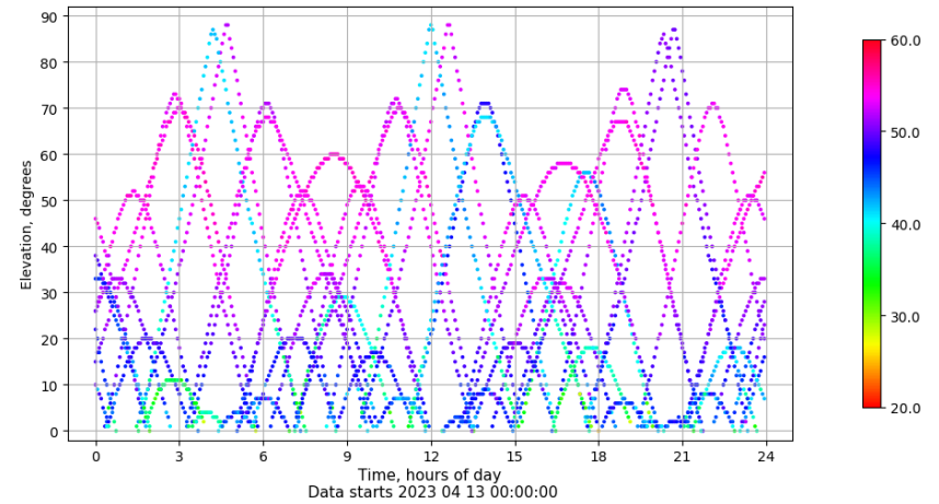
Time-elevation plot for station VALA. Signal to Noise S1C Data file VALA00ESP_R_2023103.xtr
