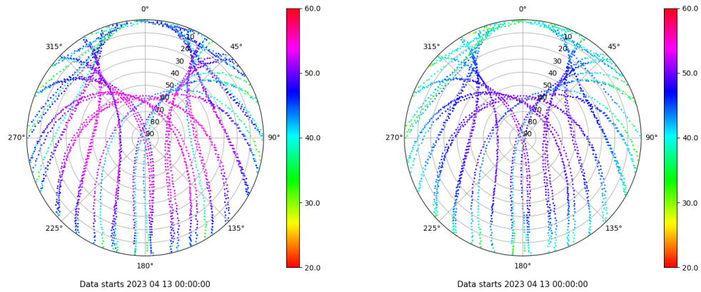
Skyplot for station VALA. Signal to Noise S1C Data file VALA00ESP_R_2023103.xtr Skyplot for station VALA. Signal to Noise S2C Data file VALA00ESP_R_2023103.xtr
