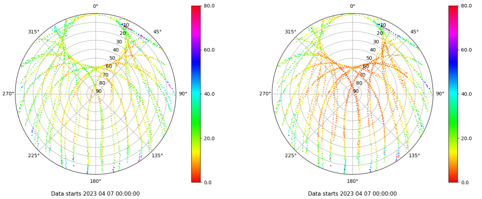
Skyplot for station VALA. Parameter M1C Data file VALA00ESP_R_2023097.xtr Skyplot for station VALA. Parameter M2C Data file VALA00ESP_R_2023097.xtr
