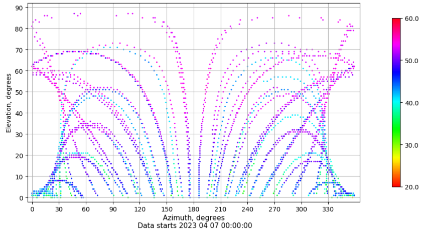
Azimuth-elevation plot for station VALA. Signal to Noise S1C Data file VALA00ESP_R_2023097.xtr
