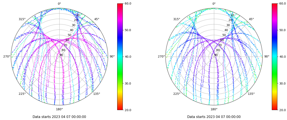
Skyplot for station VALA. Signal to Noise S1C Data file VALA00ESP_R_2023097.xtr Skyplot for station VALA. Signal to Noise S2C Data file VALA00ESP_R_2023097.xtr
