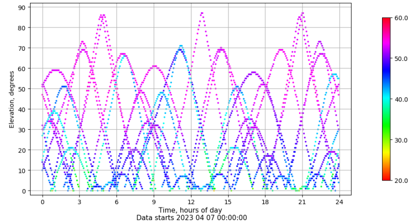
Time-elevation plot for station VALA. Signal to Noise S1C Data file VALA00ESP_R_2023097.xtr
