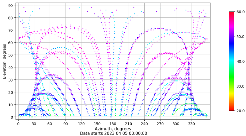
Azimuth-elevation plot for station VALA. Signal to Noise S1C Data file VALA00ESP_R_2023095.xtr
