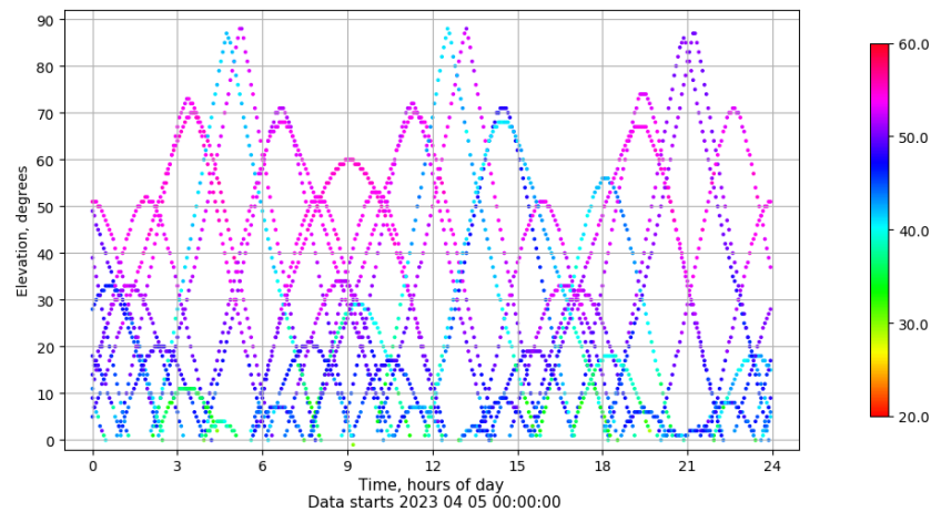
Time-elevation plot for station VALA. Signal to Noise S1C Data file VALA00ESP_R_2023095.xtr
