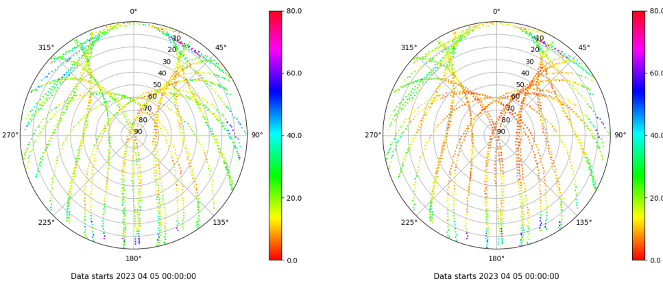
Skyplot for station VALA. Parameter M1C Data file VALA00ESP_R_2023095.xtr Skyplot for station VALA. Parameter M2C Data file VALA00ESP_R_2023095.xtr
