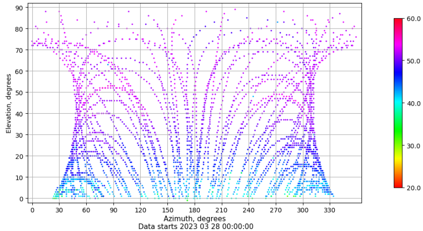
Azimuth-elevation plot for station VALA. Signal to Noise S1C Data file VALA00ESP_R_2023087.xtr
