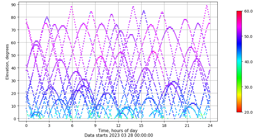
Time-elevation plot for station VALA. Signal to Noise S1C Data file VALA00ESP_R_2023087.xtr
