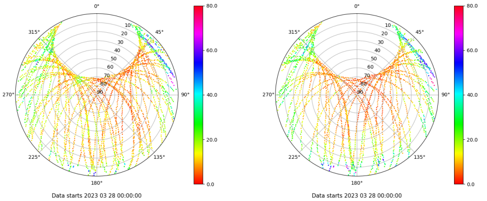
Skyplot for station VALA. Parameter M1C Data file VALA00ESP_R_2023087.xtr Skyplot for station VALA. Parameter M2S Data file VALA00ESP_R_2023087.xtr
