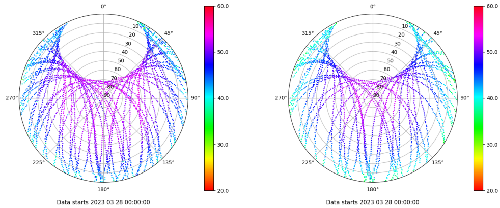
Skyplot for station VALA. Signal to Noise S1C Data file VALA00ESP_R_2023087.xtr Skyplot for station VALA. Signal to Noise S2S Data file VALA00ESP_R_2023087.xtr
