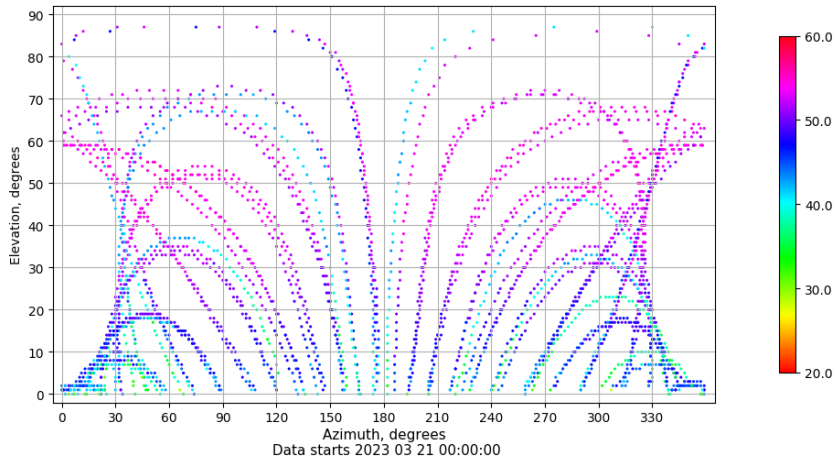
Azimuth-elevation plot for station VALA. Signal to Noise S1C Data file VALA00ESP_R_2023080.xtr
