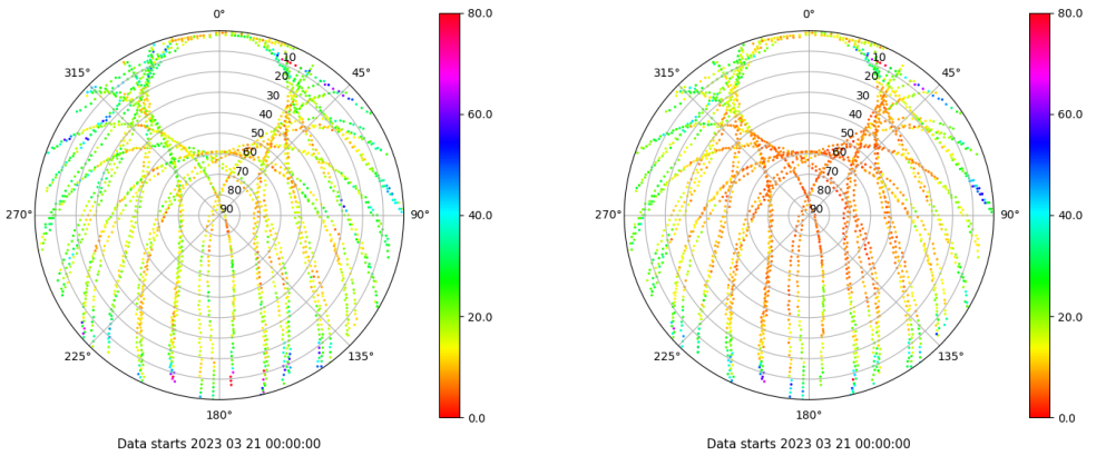
Skyplot for station VALA. Parameter M1C Data file VALA00ESP_R_2023080.xtr Skyplot for station VALA. Parameter M2C Data file VALA00ESP_R_2023080.xtr
