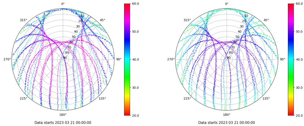
Skyplot for station VALA. Signal to Noise S1C Data file VALA00ESP_R_2023080.xtr Skyplot for station VALA. Signal to Noise S2C Data file VALA00ESP_R_2023080.xtr
