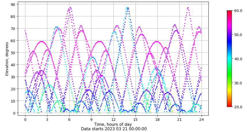
Time-elevation plot for station VALA. Signal to Noise S1C Data file VALA00ESP_R_2023080.xtr
