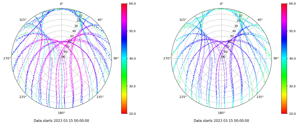
Skyplot for station VALA. Signal to Noise S1C Data file VALA00ESP_R_2023074.xtr Skyplot for station VALA. Signal to Noise S2C Data file VALA00ESP_R_2023074.xtr
