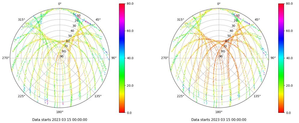
Skyplot for station VALA. Parameter M1C Data file VALA00ESP_R_2023074.xtr Skyplot for station VALA. Parameter M2C Data file VALA00ESP_R_2023074.xtr
