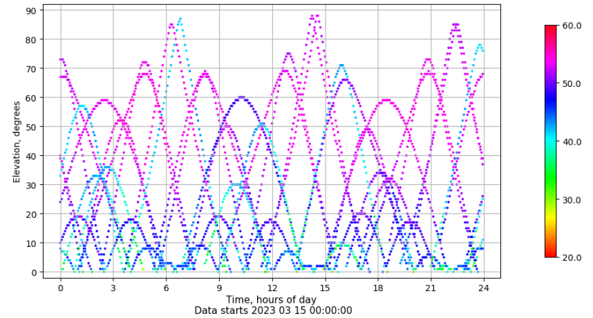
Time-elevation plot for station VALA. Signal to Noise S1C Data file VALA00ESP_R_2023074.xtr
