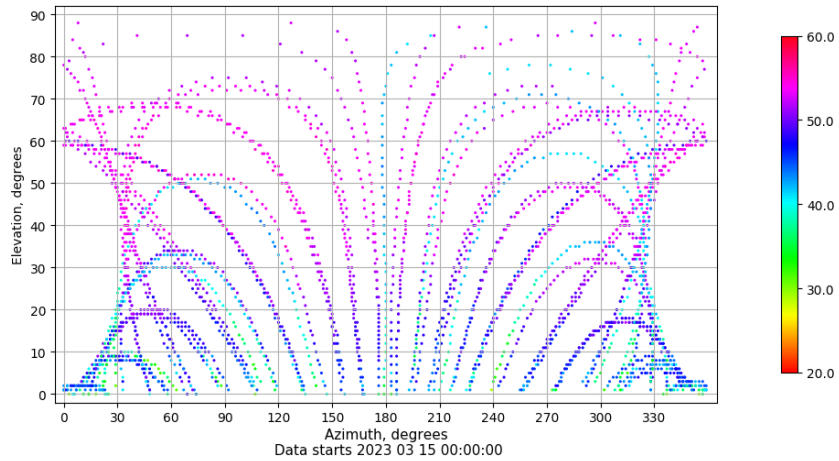
Azimuth-elevation plot for station VALA. Signal to Noise S1C Data file VALA00ESP_R_2023074.xtr
