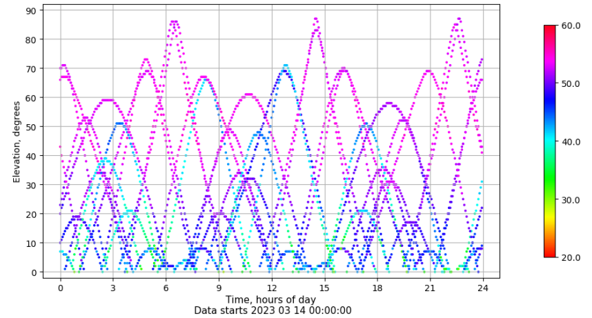
Time-elevation plot for station VALA. Signal to Noise S1C Data file VALA00ESP_R_2023073.xtr
