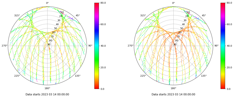
Skyplot for station VALA. Parameter M1C Data file VALA00ESP_R_2023073.xtr Skyplot for station VALA. Parameter M2C Data file VALA00ESP_R_2023073.xtr
