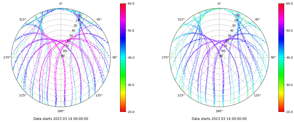
Skyplot for station VALA. Signal to Noise S1C Data file VALA00ESP_R_2023073.xtr Skyplot for station VALA. Signal to Noise S2C Data file VALA00ESP_R_2023073.xtr
