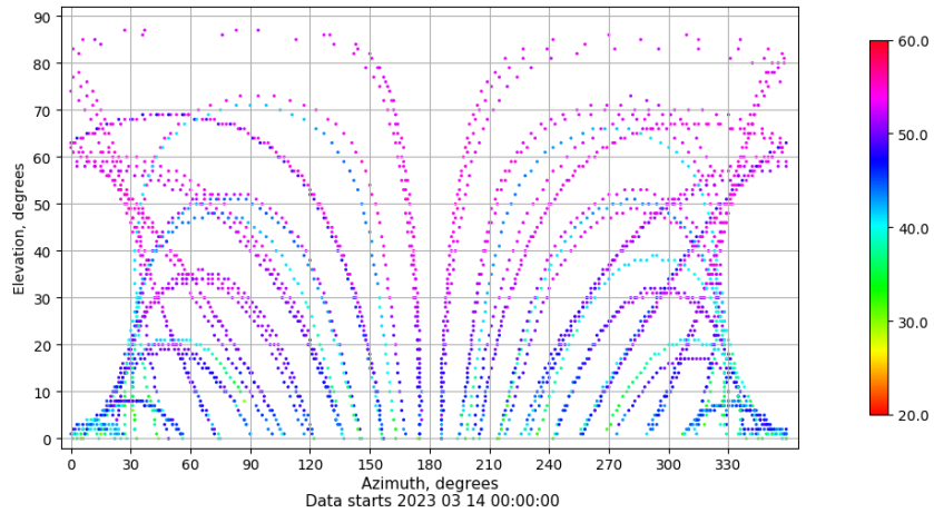
Azimuth-elevation plot for station VALA. Signal to Noise S1C Data file VALA00ESP_R_2023073.xtr
