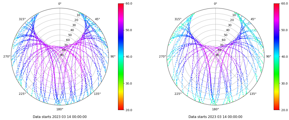
Skyplot for station VALA. Signal to Noise S1C Data file VALA00ESP_R_2023073.xtr Skyplot for station VALA. Signal to Noise S2S Data file VALA00ESP_R_2023073.xtr
