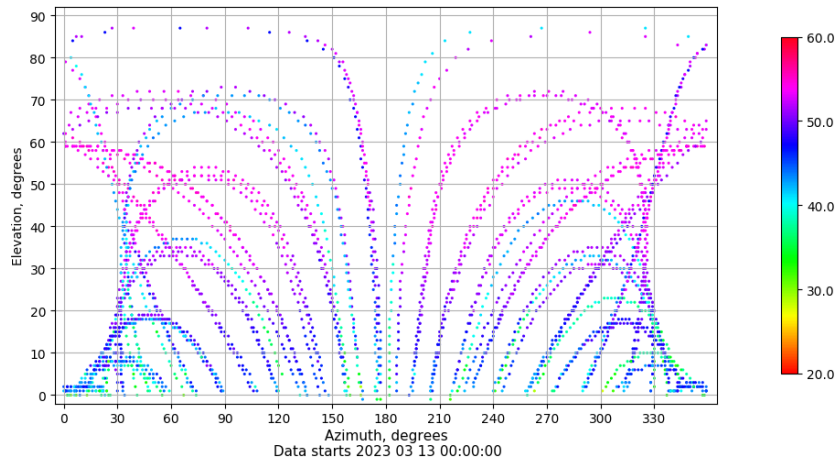
Azimuth-elevation plot for station VALA. Signal to Noise S1C Data file VALA00ESP_R_2023072.xtr
