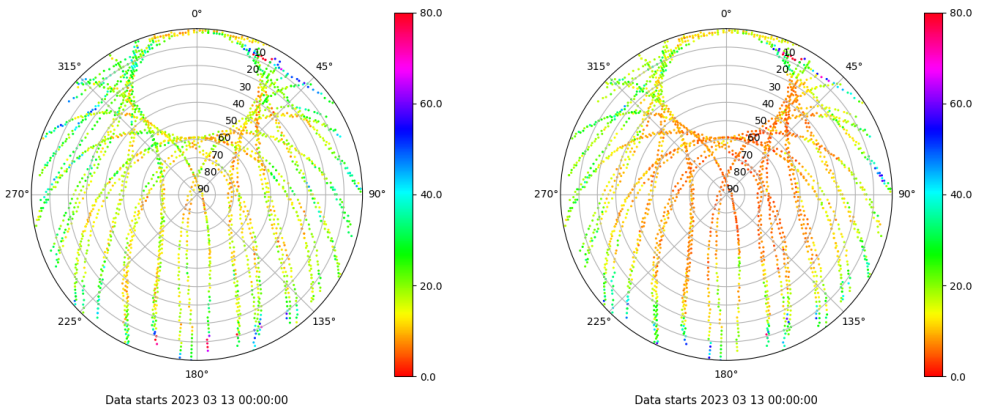
Skyplot for station VALA. Parameter M1C Data file VALA00ESP_R_2023072.xtr Skyplot for station VALA. Parameter M2C Data file VALA00ESP_R_2023072.xtr
