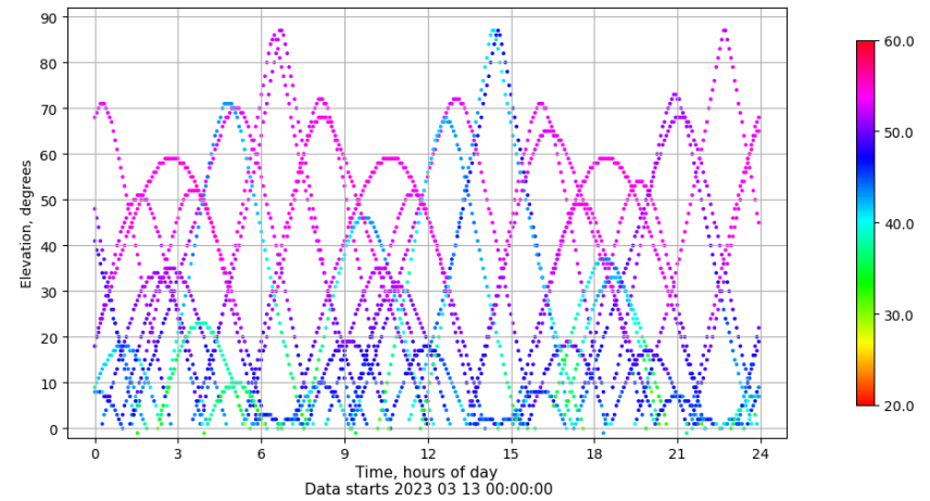
Time-elevation plot for station VALA. Signal to Noise S1C Data file VALA00ESP_R_2023072.xtr
