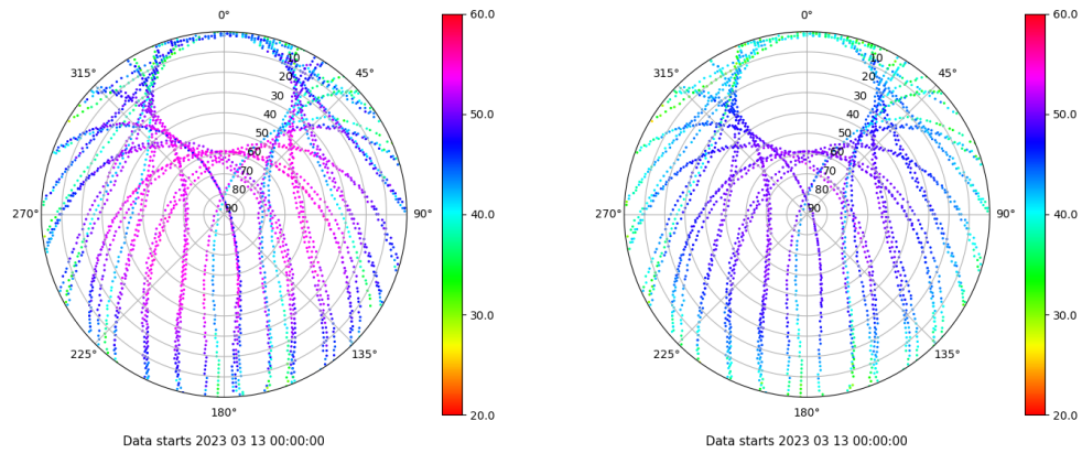
Skyplot for station VALA. Signal to Noise S1C Data file VALA00ESP_R_2023072.xtr Skyplot for station VALA. Signal to Noise S2C Data file VALA00ESP_R_2023072.xtr
